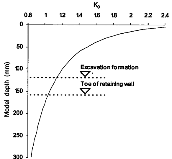
Fig. 11 Variation of K_0 with depth over depth of model
