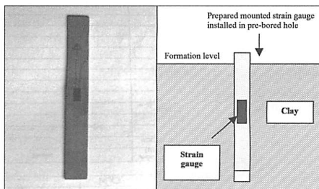
Fig. 8 Strain gauged insert for instrumented heave reducing piles
