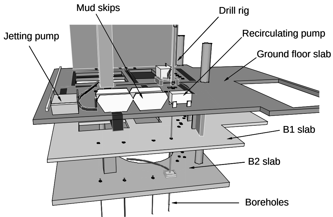
Figure 3 Schematic showing dewatering and instrumentation installation on site.
