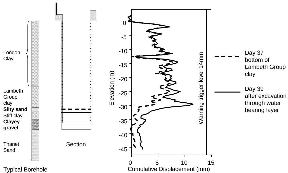
Figure 15 Inclinator data reflecting the movement associated with excavation through water bearing layer in the Upper Lambeth Group.
