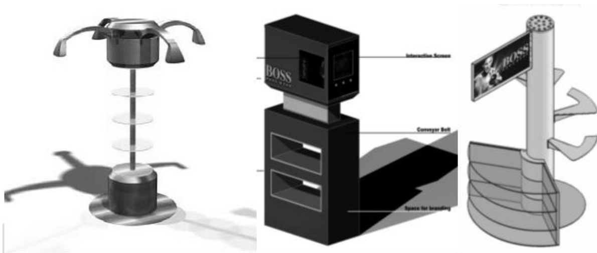
Figure 3 Designs of some of the prototypes
