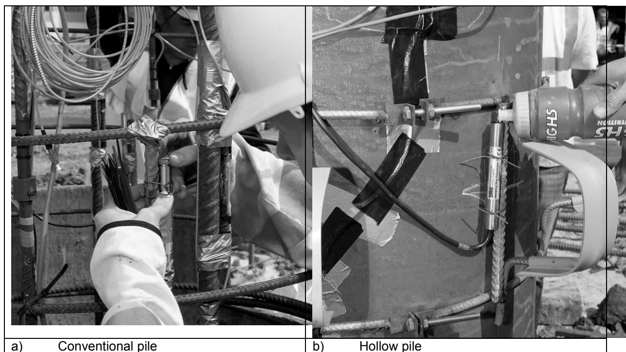
Figure 7 Filing vibrating wire piezometers with water
