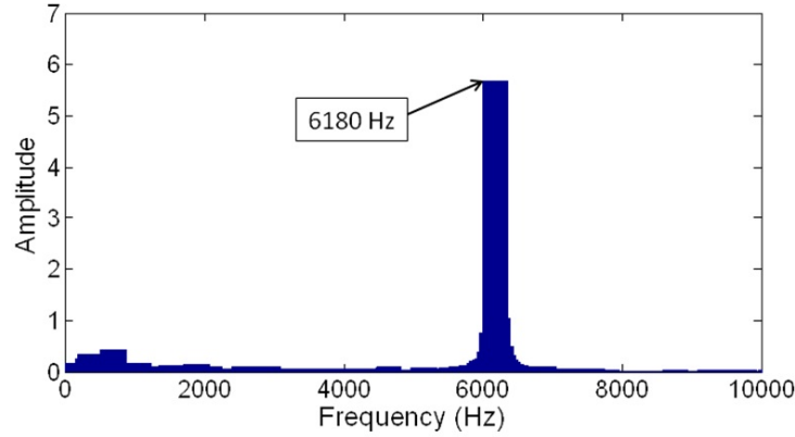
Figure 11: Fourier transform components from one of the numerical sensors on the casing
