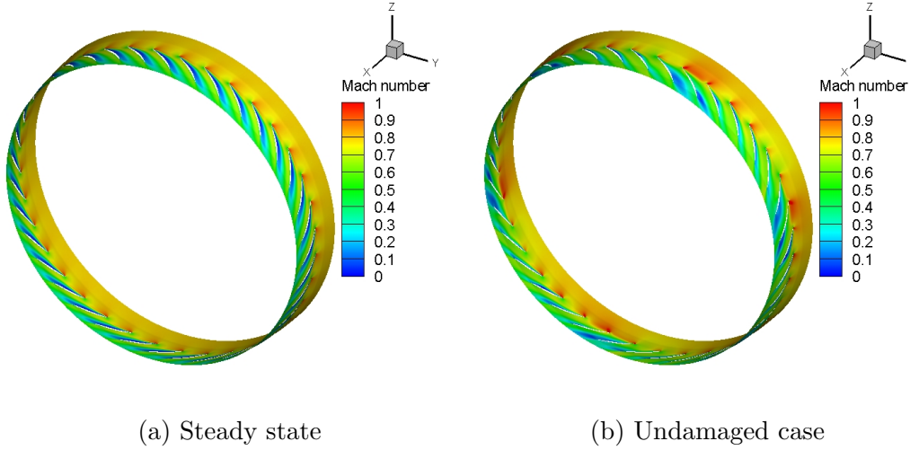
Figure 15: Mach number contour comparison at 75% span of the rotor
