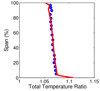
Figure 9: Total pressure ratio and temperature ratio distributions downstream of rotor, at high flow conditions (Blue: experimental data; Red: CFD solutions)
