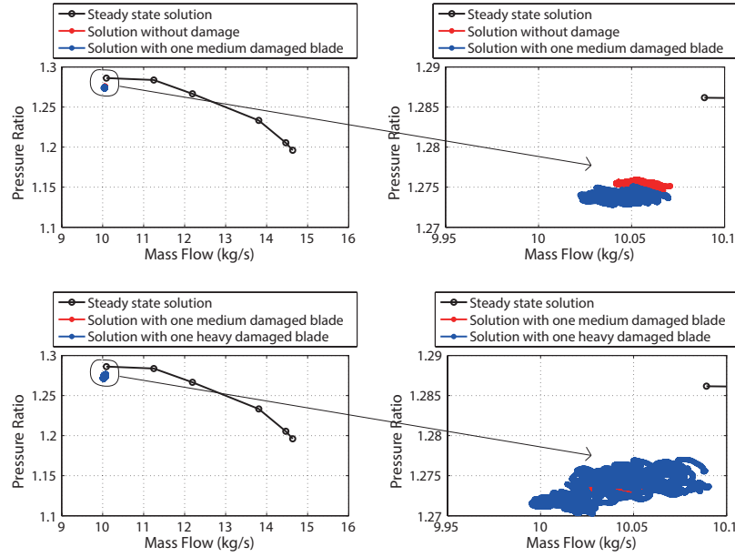
Figure 21: Compressor performance during rotating stall with one damaged blade
