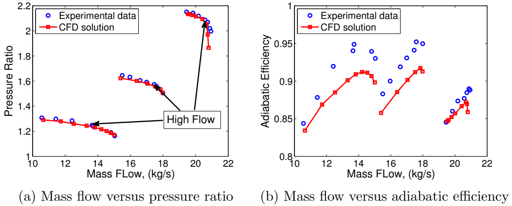
Figure 8: Compressor map comparisons (Right to left: design speed, 80% speed and 60% speed)
