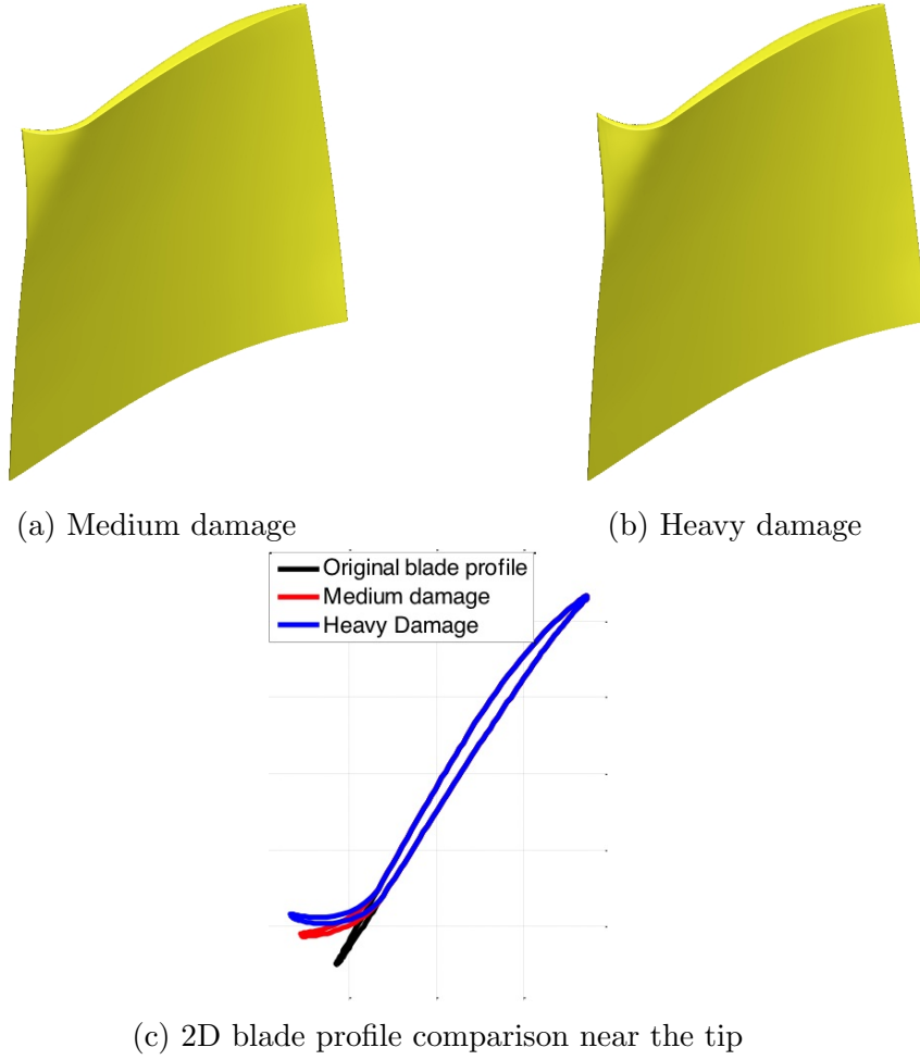
Figure 12: Curl damage at leading edge
