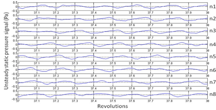
(b) Time history in one rotor revolution for Damaged Case 2
