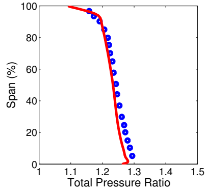
Figure 9: Total pressure ratio and temperature ratio distributions downstream of rotor, at high flow conditions (Blue: experimental data; Red: CFD solutions)
