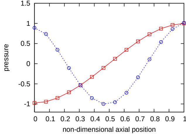
Fig. 6. Numerical prediction of the first two fundamental pressure mode shapes due to randomly vibrating wall for L = 405.5 mm (— 1 st axial mode ( f^{1A} = 419 Hz); - - - 2 nd axial mode ( f^{2A} = 838 Hz))
