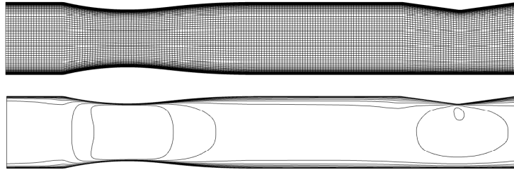
Fig. 12. Computational grid of the Déclery B nozzle ( Ni \times Nj = 201 \times 101 ) and steady Mach number for an inlet flow velocity u_0 = 17\text{ms}^{-1}
