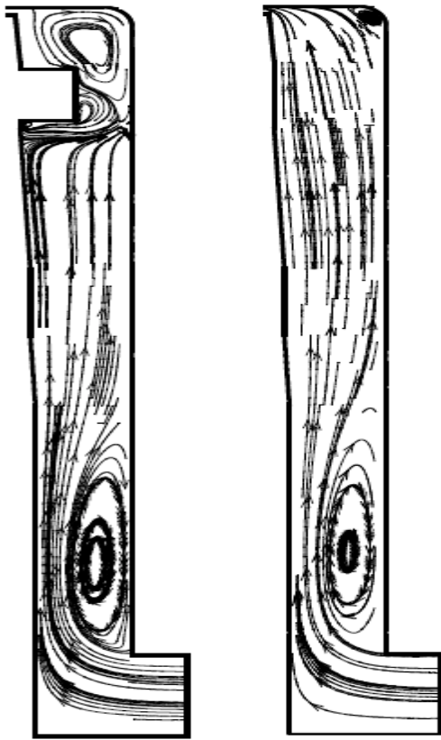
Figure 22. Velocity Streamlines for Re_\tau = 6.8 \times 10^6 and C_w = 10^5 .
