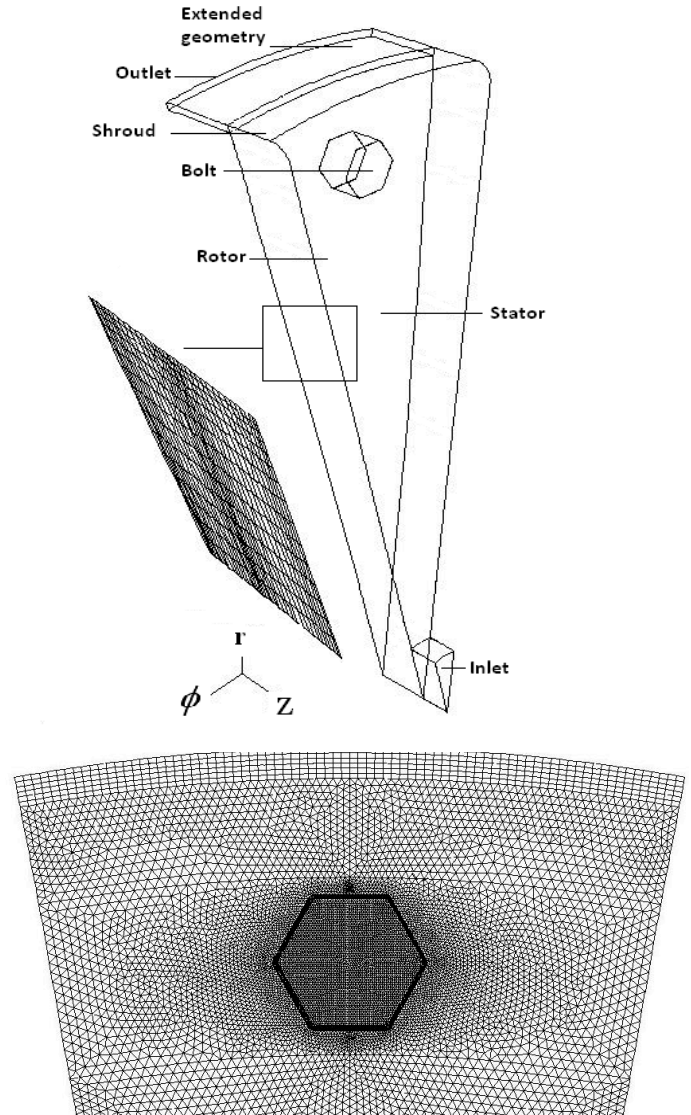
Figure 14. A Section of the Computational Mesh used for the Bolt Windage Test Rig
