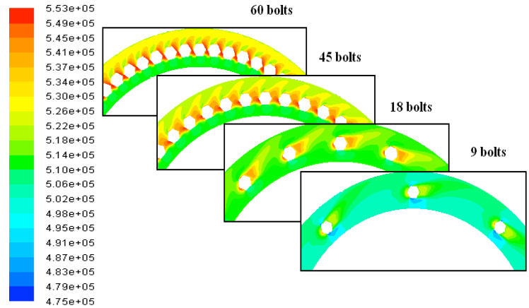
Figure 20. Total pressure Contours around the Bolts for N = 9, 18, 45 and 60 ( Re = 6.8 \times 10^6 and C_w = 10^5 ).
