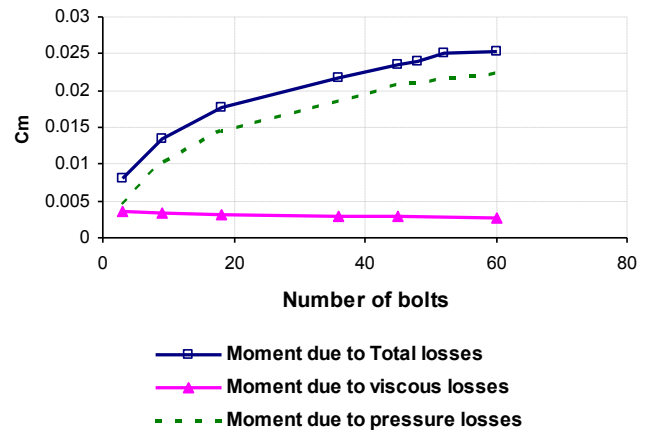
Figure 21. Variation of viscous losses, pressure losses, and total losses with different number of bolts ( Re = 6.8 \times 10^6 and C_w = 10^5 ).
