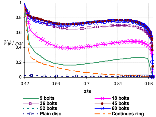
Figure 17. Predicted Axial Variation of Dimensionless Tangential Velocity at r/b = 0.9 , Re_c = 6.8 \times 10^6 and C_w = 10^5 ( \lambda_T = 0.35 ).
