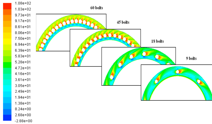
Figure 19. Tangential velocity Contours around the Bolts for N = 9, 18, 45 and 60 ( Re = 6.8 \times 10^6 and C_w = 10^5 ).
