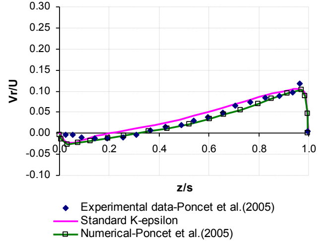
Figure 12. Axial Variation of Radial Velocity at r/b = 0.8 .
