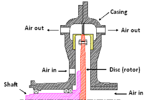
Figure 1. Schematic Diagram of the Bolt Windage Test Rig
