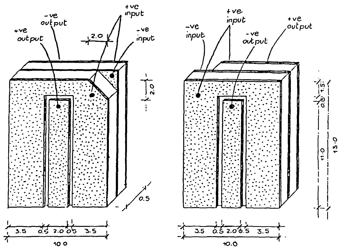
Figure 4.3.3 Electrical connections for self monitoring transmitter element.
