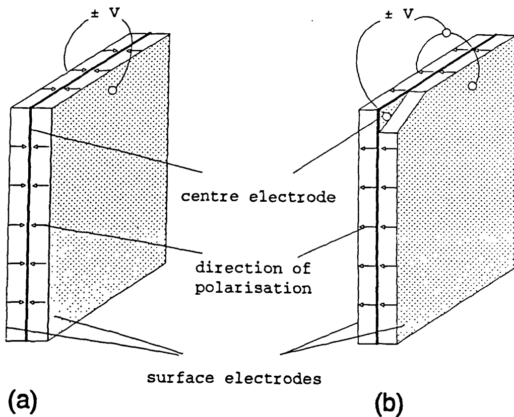
Figure 4.3.2 Electrical connections for bender elements. (a) series connected (b) parallel connected.
