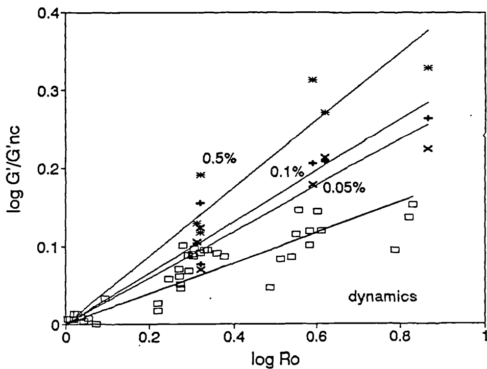
Figure 5.7.15 Speswhite kaolin. Tests LSK1 to LSK10. Dependence of tangent stiffness on overconsolidation ratio at different shear strain amplitudes
