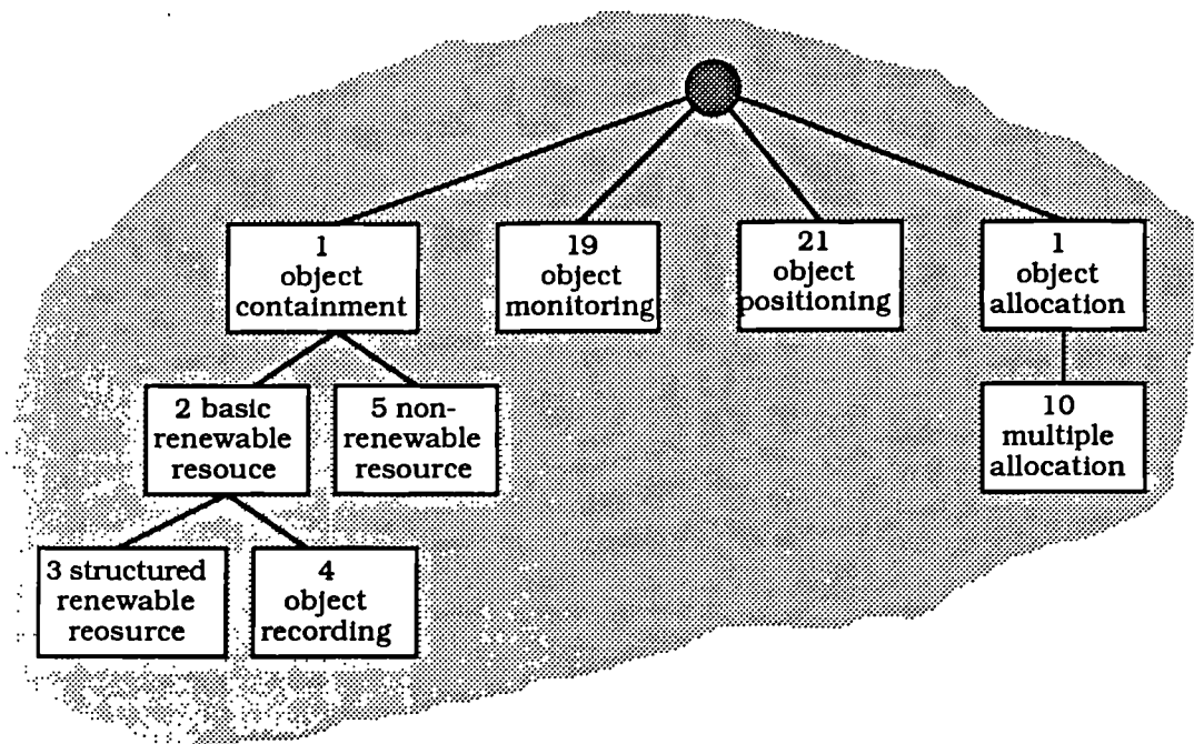
Domain abstraction hierarchy implemented by the prototype version of Ira
