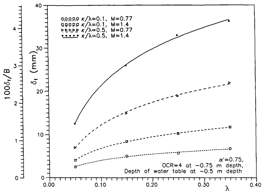
Figure 7.23 Variations of settlement \delta_f and settlement ratio 100\delta_f/B at failure with \lambda for fixed values of \kappa/\lambda , M and \alpha'
