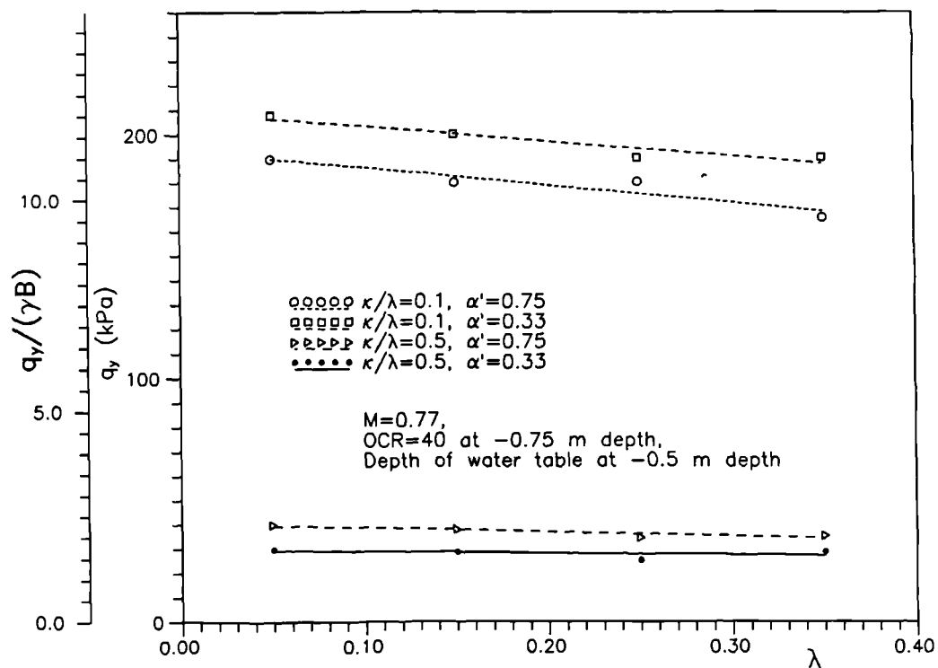
Figure 7.22 Variations of bearing pressure q_y and normalised bearing pressure q_y/(\gamma B) immediately after yield with \lambda for fixed values of \kappa/\lambda , M and \alpha'
