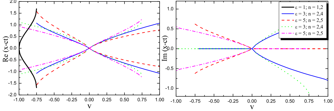
Figure 1: (x-ct) as a function of v for \varepsilon = 1, 3, 5 for some particular branches.
