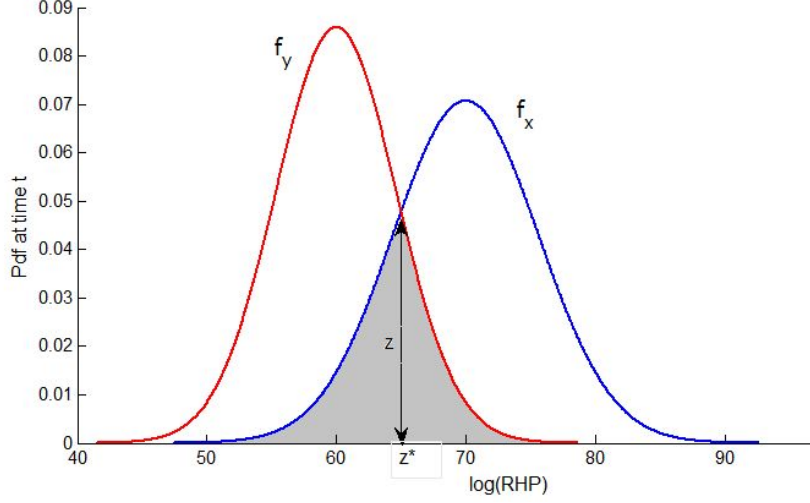
Fig. 1: Probability distributions functions of the RHP of two individuals at time t . The shaded area describes the overlap between the two distributions.
