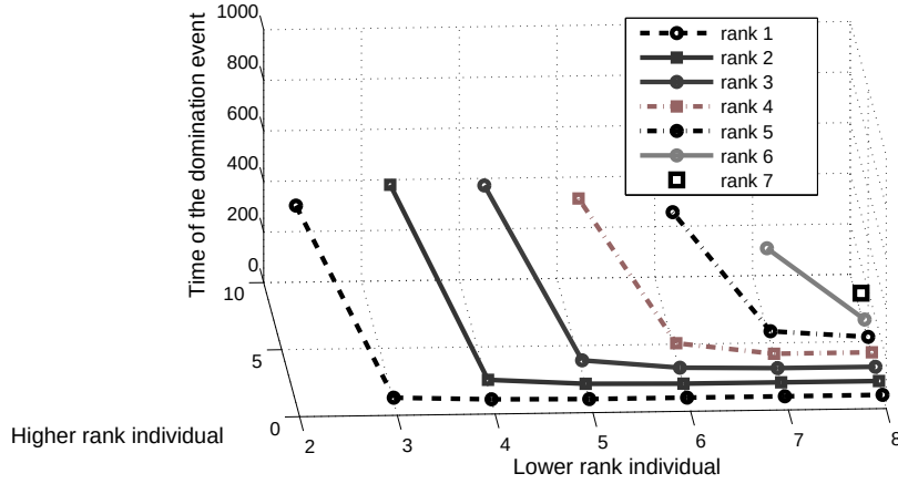
Fig. 10: The time of domination events between each pair of individuals in the updated model (e.g., the black dashed line representing rank1, shows the time of domination event of the first rank individual with ranks 2,3,4,5,6,7,8) for \theta = 1 , W = 0.1 , L = 0 , N = 8 and perfect estimation:
