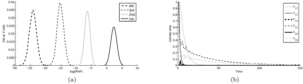
Fig. 8: a) Probability distribution functions of RHP for the 4 individuals in the updated model: t = 500 , only L is present. b) \nu_{xy} over time when only L is present. \nu_{14}(t) coincides with the x -axis after t = 1 .
