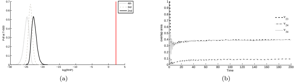
Fig. 4: a) Probability distribution for the second, third, forth place individuals for W = 0 and L = 0.1 at t = 500 . The first place does not have a distribution as it's RHP stays unchanged and is represented by the vertical line ( x = \log(10) ) b) Time course of the corresponding area of overlap \nu_{xy}(t) , x = 2, 3, 4, y = 3, 4 . \nu_{23}(t) and \nu_{34}(t) overlap with each other. The overlap between the top individual and the other individuals becomes close to 0 very quickly.
