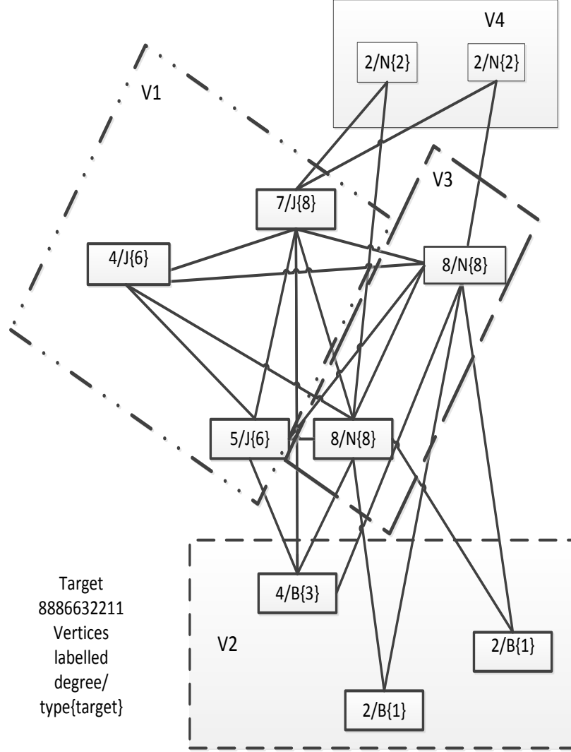
FIGURE 1. A minimal graph for the target 8886632211 separating the Joiners V1, the Breakers V2, Neutrals joined to at least one Breaker and thus all Joiners V3, and Neutrals not joined to any Breaker V4. The numbering is as in Theorem 7; there is no set V5.
