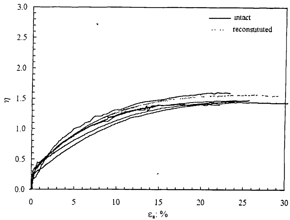
Figure 5.16 Shear behaviour of reconstituted and intact samples of calcarenite which yielded in isotropic compression (constant p' tests).
