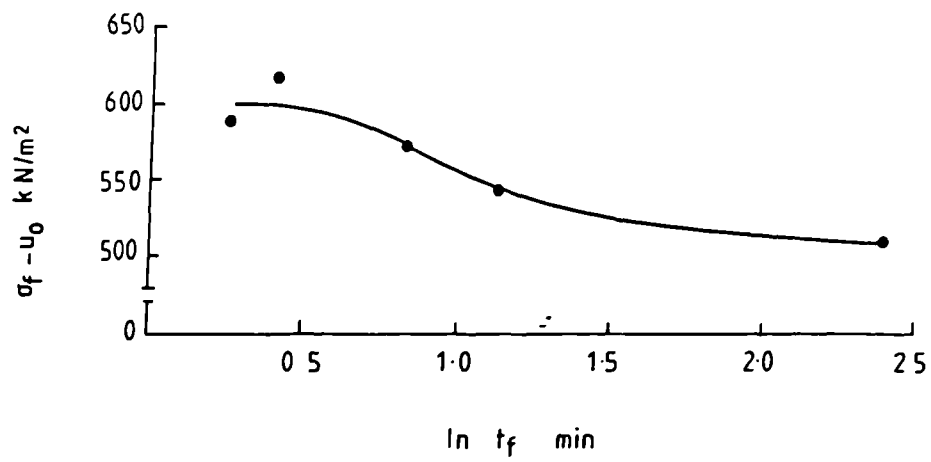
Fig 10.19 EFFECT OF TIME TO FAILURE ON \sigma_f - \sigma_u : GROUP F-3
