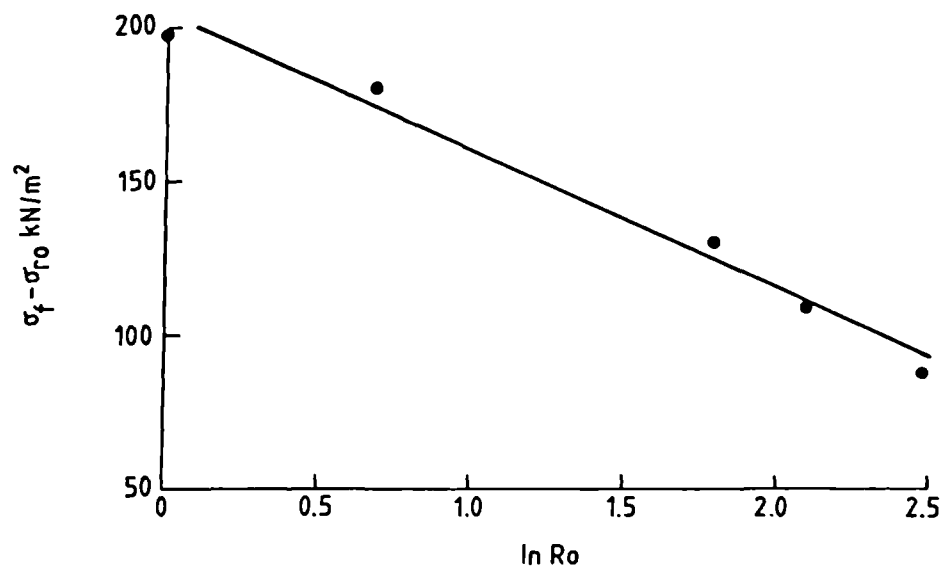
Fig 10.15 PLOT OF \sigma_f - \sigma_{r0} AGAINST \ln R_0 : GROUP F-5
