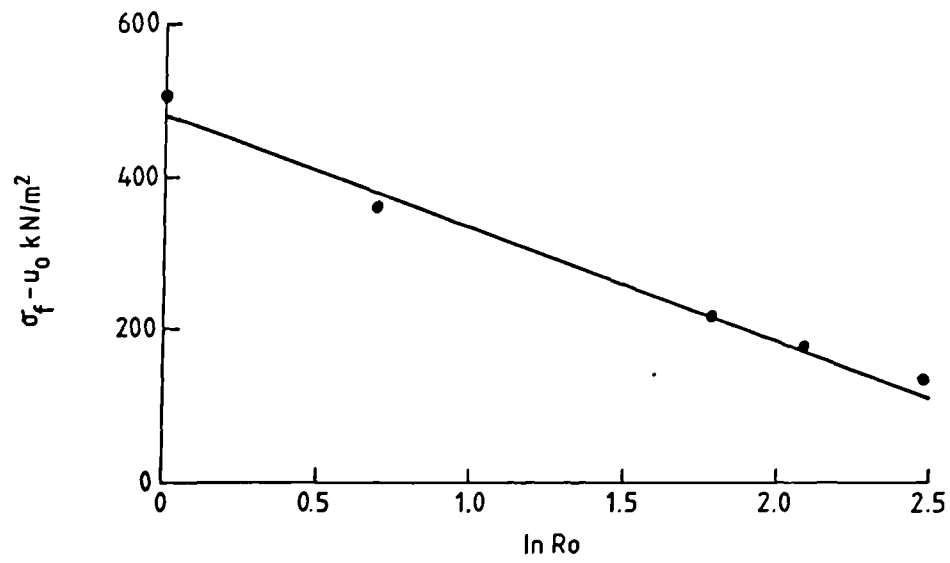
Fig 10.14 PLOT OF \sigma_f - u_0 AGAINST \ln R_0 : GROUP F-5
