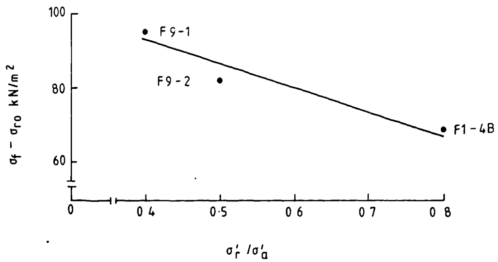
Fig 10.30 EFFECT OF STRESS RATIO \sigma'_r/\sigma'_a ON \sigma_f - \sigma_{ro} GROUP F-9
