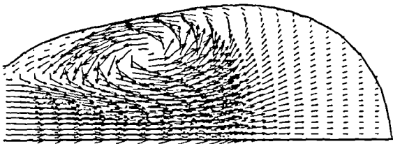
Figure 1. Flow at T = 480 \text{ ms}
