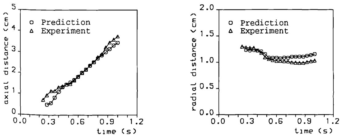
Figure 7.47 Vortex centre trajectories for Case I
