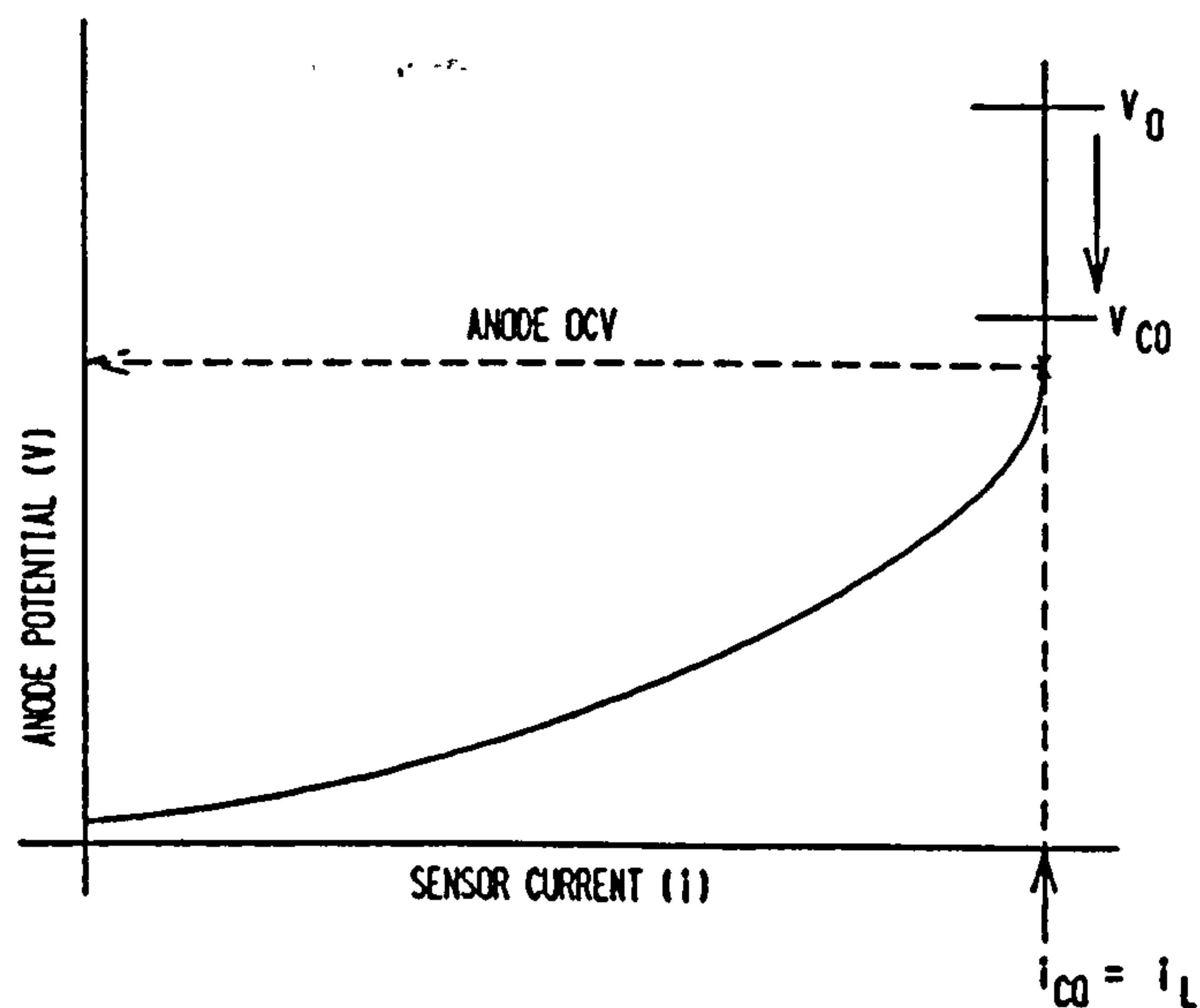
Figure 11 Schematic diagram showing anode polarization under load. [After CTL Report No. 81/31/006, (2) 12 p.7]
