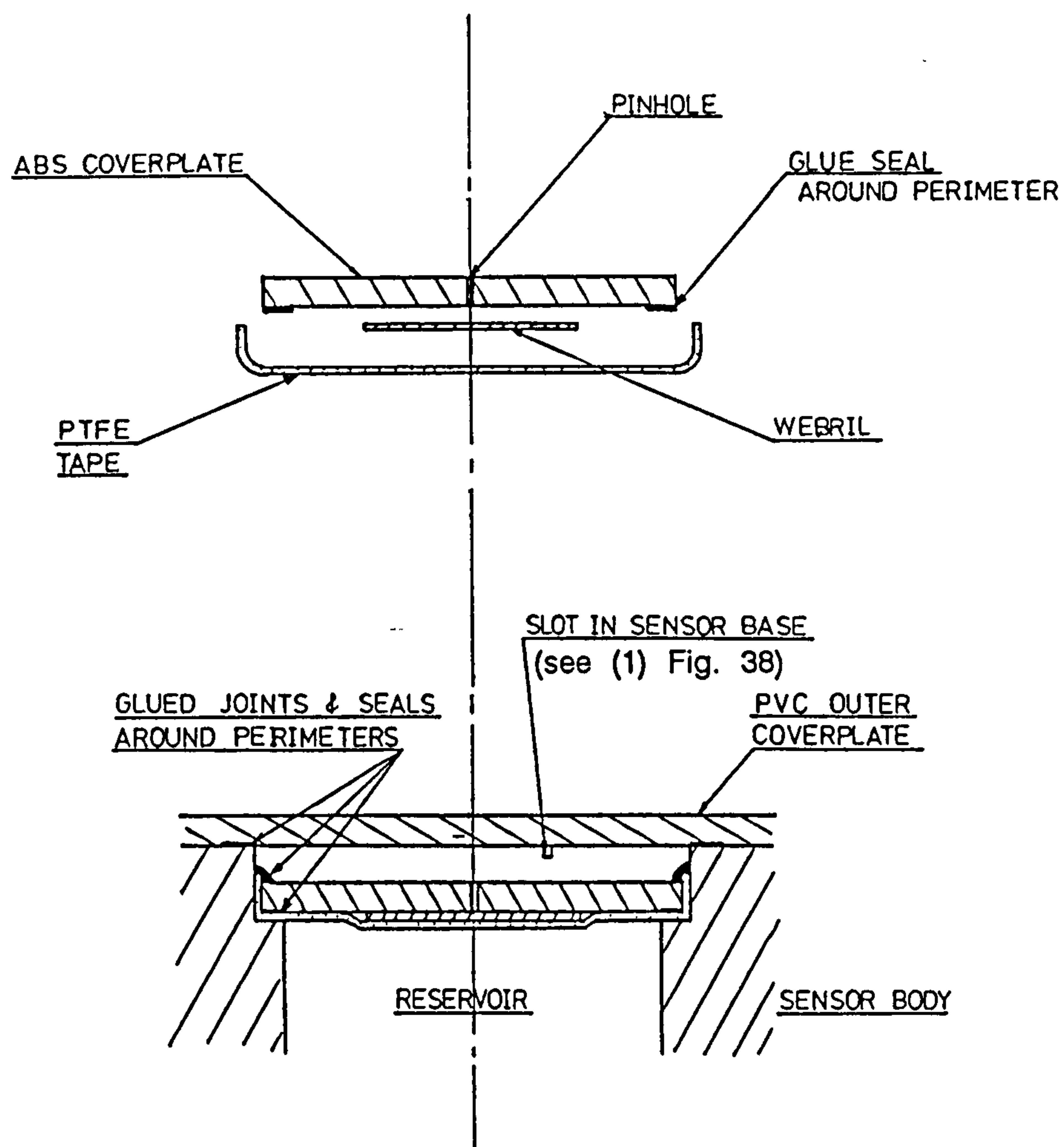
Figure 37 Schematic drawing of the Pressure Release System & Rear Coverplate Seal Design [After CTL Report No. 82/09/007, (2) 13 Fig. 2.5]
