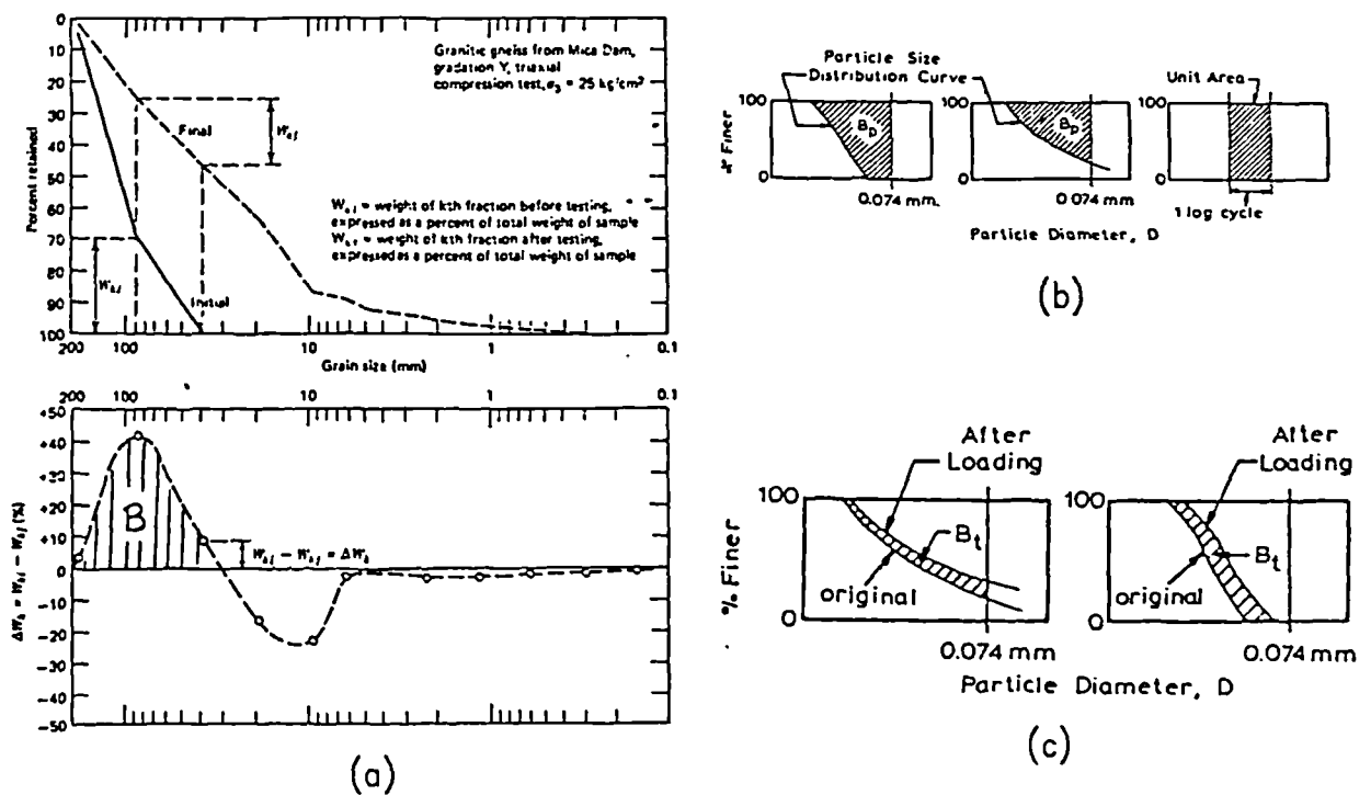
Figure 4.28 Particle crushing measurement
