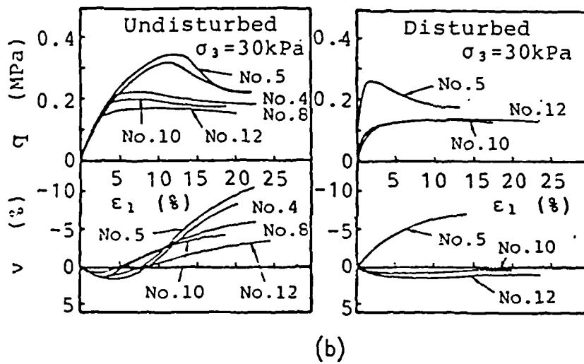
Figure 4.21 Comparison of stress-strain curves for undisturbed and disturbed samples (a) (after Yagi and Yatabe, 1985) (b) (after Murata and Yasufuku, 1987)
