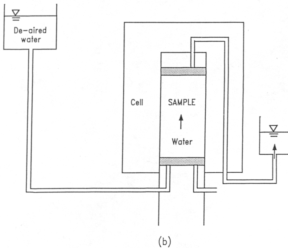
Figure 5.14 Sample saturation arrangement (a) \text{CO}_2 circulation (b) De-aired water circulation
