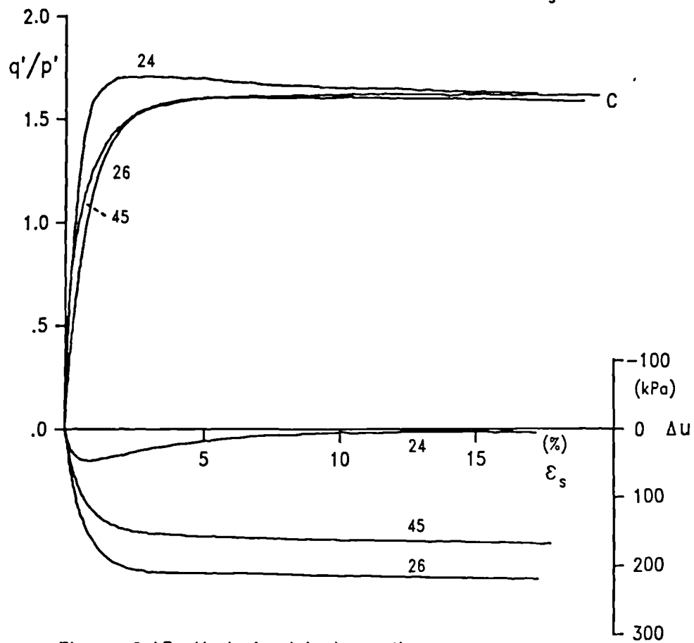
Figure 6.15 Undrained test results
