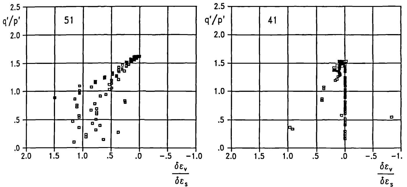
Figure 6.24 Stress-dilatancy of compacted and over-consolidated samples
