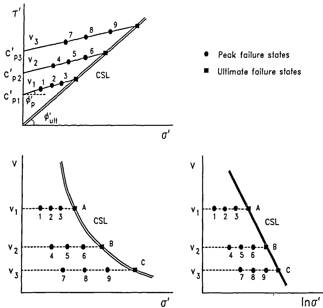
Figure 3.5 Failure states (Coulomb-Hvorslev model)
