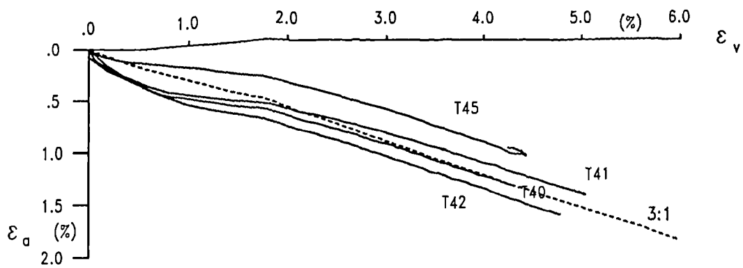
Figure 6.10 \varepsilon_v - \varepsilon_a during isotropic compression
