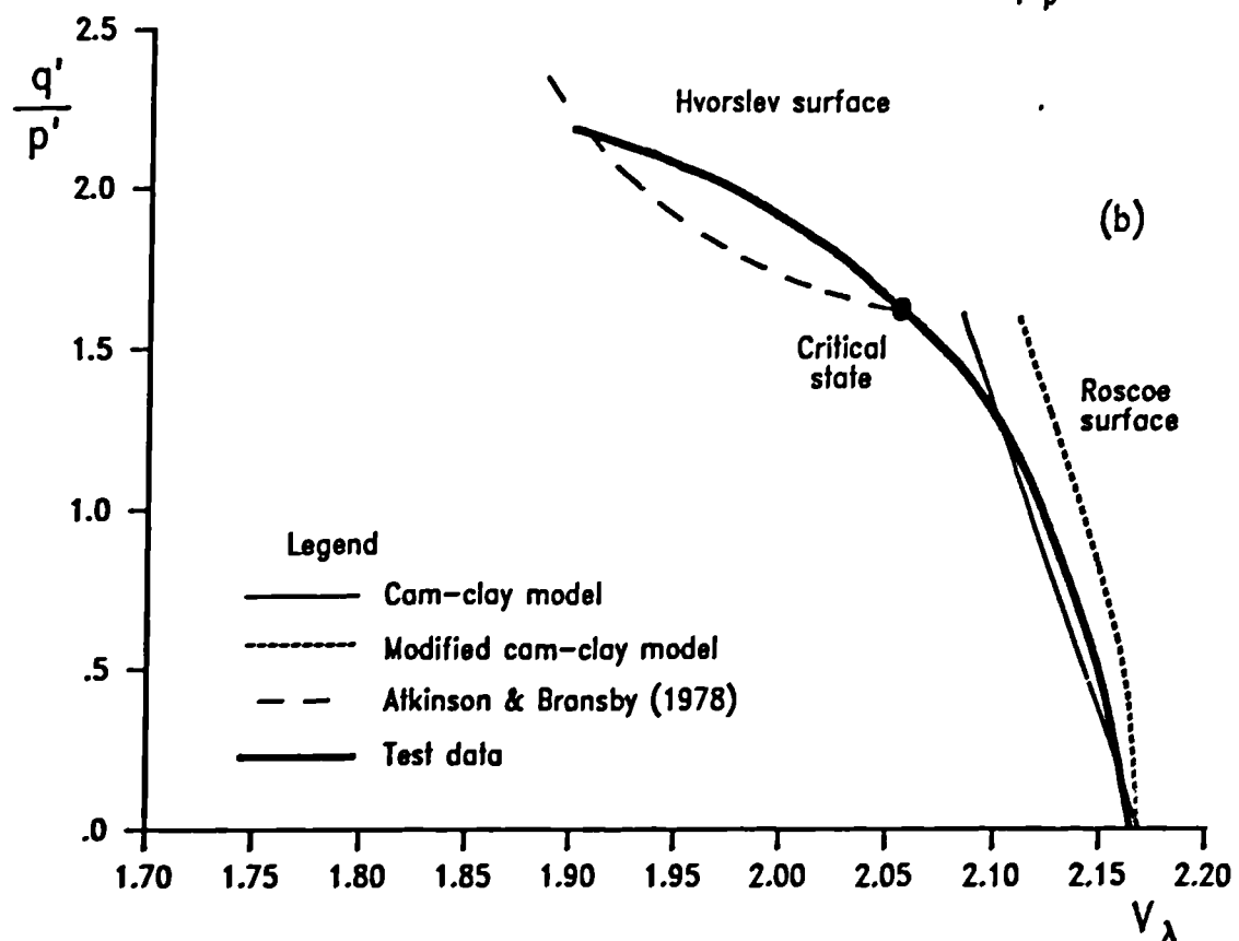
Figure 6.34 Comparison with Cam-clay soil models
