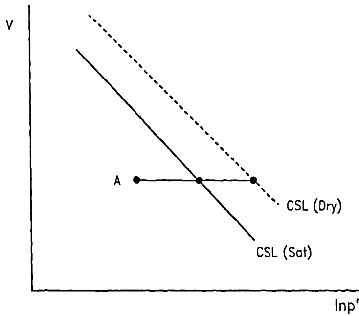
Figure 6.51 Current state in v: \ln p' space
