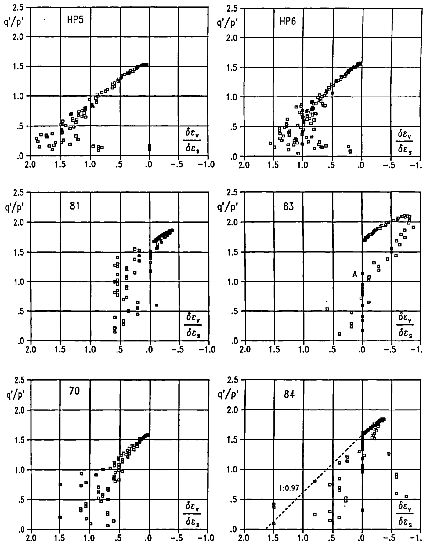
Figure 6.22 Stress-dilatancy relationships
