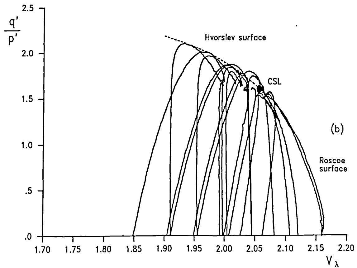
Figure 6.33 Normalised stress paths (drained tests)
