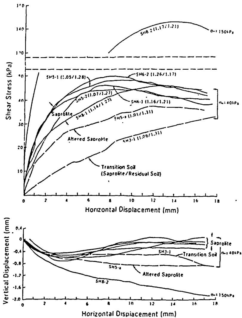
Figure 4.20 Stress-deformation curves for various decomposed granite soils (after Irfan, 1985)
