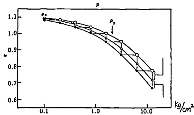
Figure 4.17 Oedometer test on undisturbed decomposed granite soil (after JSSMFE, 1979)
