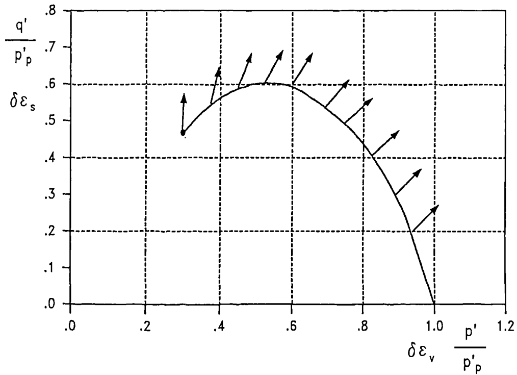
Figure 6.35 Strain increment vectors for test HP6
