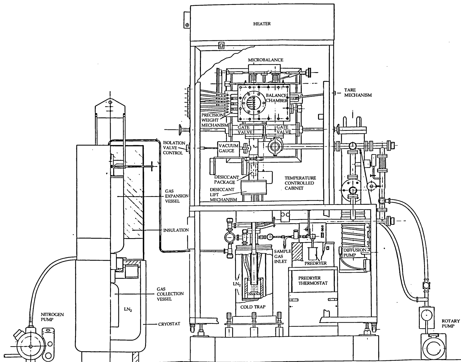
Figure 7 General assembly drawing of the gravimetric hygrometer (Forton and Pragnell, 1985)
