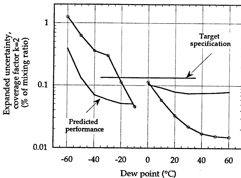
Figure 23 Comparison of the uncertainty of the gravimetric hygrometer (†) with the target specification for the humidity facility, and with the predicted performance of the hygrometer
