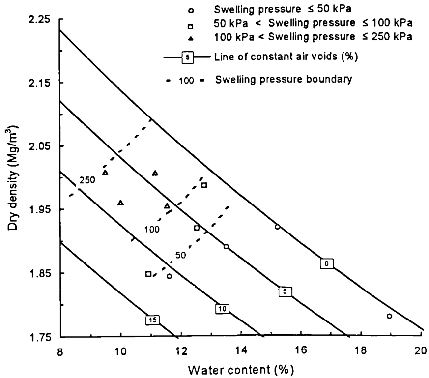
Figure 6.9 Initial state of soil with ranges of net swelling pressure - Brickearth, 100 mm cell.
