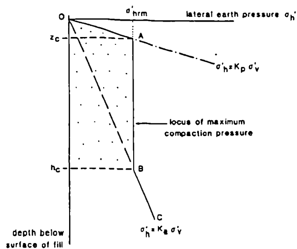
Figure 2.45 Simplified lateral stress distribution (after Ingold, 1979).
