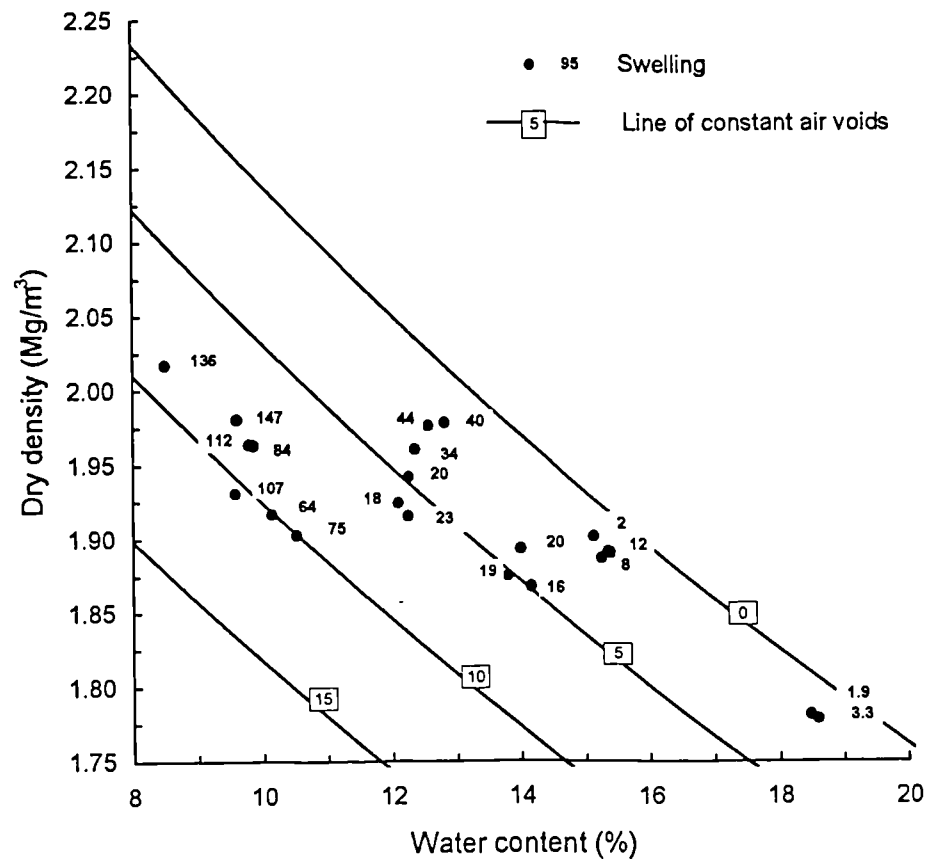
Figure 6.4 state of soil with values of net swelling pressure - Bricearth, modified oedometer.
