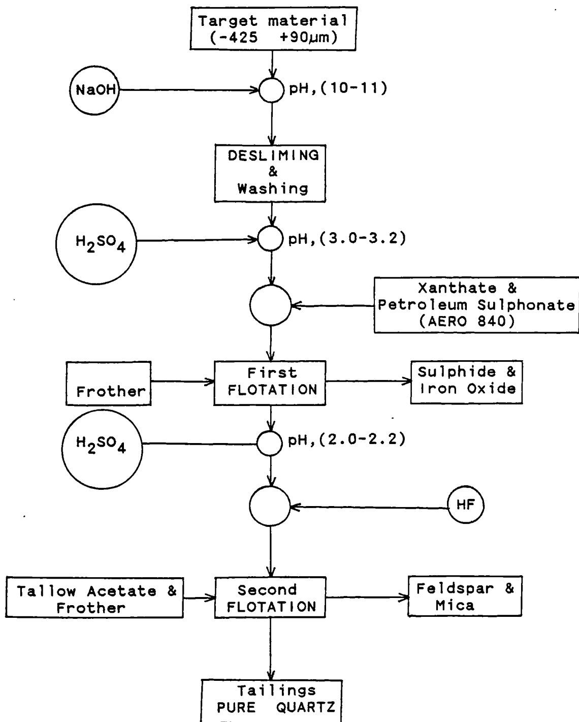
FIGURE 6.15 Schematic flowsheet of flotation process.
