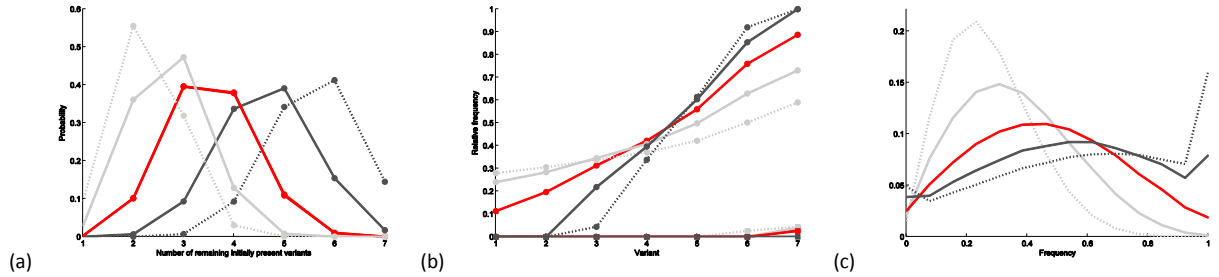
Figure 2. (a) Probability distribution P(K(50) = l | X_0, \mathbb{H}) with X_0 = [1 \ 2 \ 5 \ 10 \ 20 \ 40 \ 60] under the assumption of neutral evolution (red lines), conformity ( b = -0.002 (dark grey solid line), b = -0.004 (dark grey dashed line)) and anti-conformity ( b = 0.002 (light grey solid line), b = 0.004 (light grey dashed line)) (b) corresponding 95% confidence intervals of the possible frequency ranges for each variant (c) corresponding probability distribution P(X_7(50) | X_0, \mathbb{H}) of variant 7 after t=50 time steps. The distributions P(X_i(t) | \mathbf{y}_0, \mathbb{H}) under the considered selection hypotheses \mathbb{H} are obtained by using simulations and averaging over 100,000 runs.
