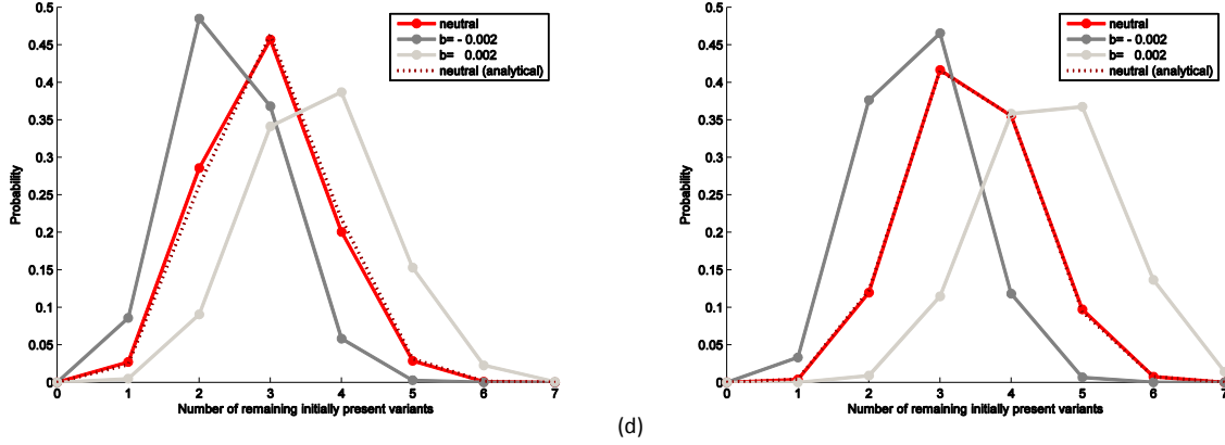
Figure 1. Probability distributions of the number of remaining initially present variants ( X_0=[1\ 2\ 5\ 10\ 20\ 40\ 60] )
