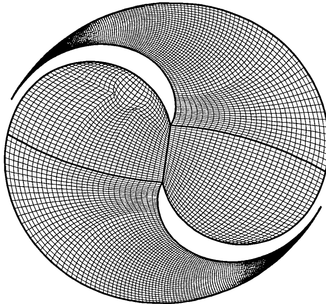
Figure 4.62 Grid 150*30*1. (Refined mesh) Crank angle 930^0 , Non Uniform Distribution, Circular arcs, Inlet pipe diameter 0.01 (smaller pipe diameter)
