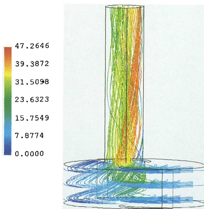
Figure 5.107 Scroll-Compressor. Rotational speed 3000 RPM, Stream lines, step=100, 50 degrees (2.777m sec) after discharge commences
