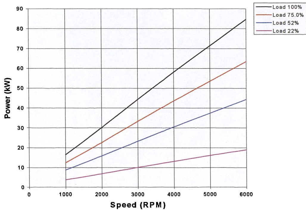
Figure 3.24 Power / Speed. Working fluid R134A wet vapour. Different Load conditions.
