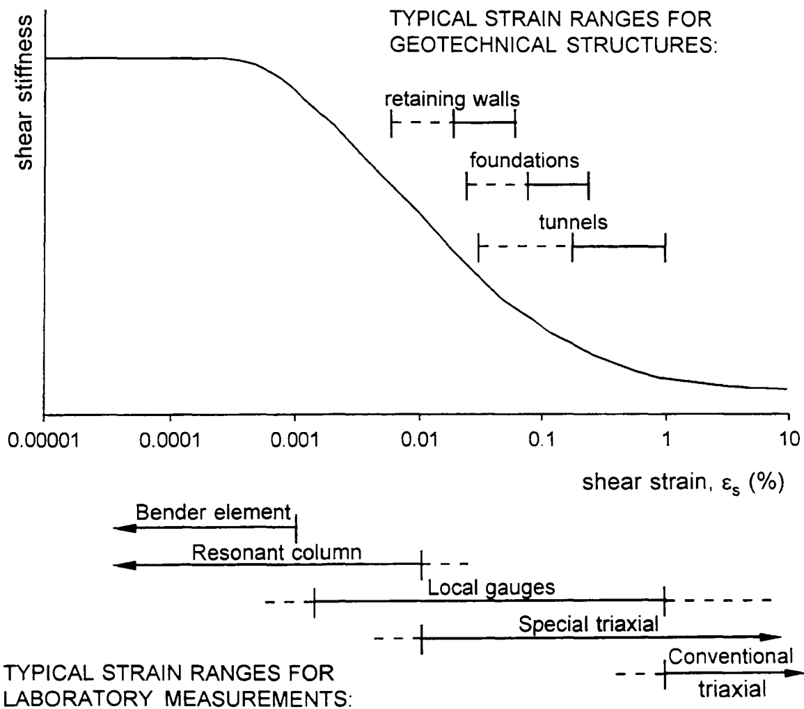
Figure 2.5 Approximate strain limits for reliable measurement of soil stiffness (after Atkinson and Sallfors, 1991) and typical strain ranges for geotechnical structures (after Mair, 1993)
