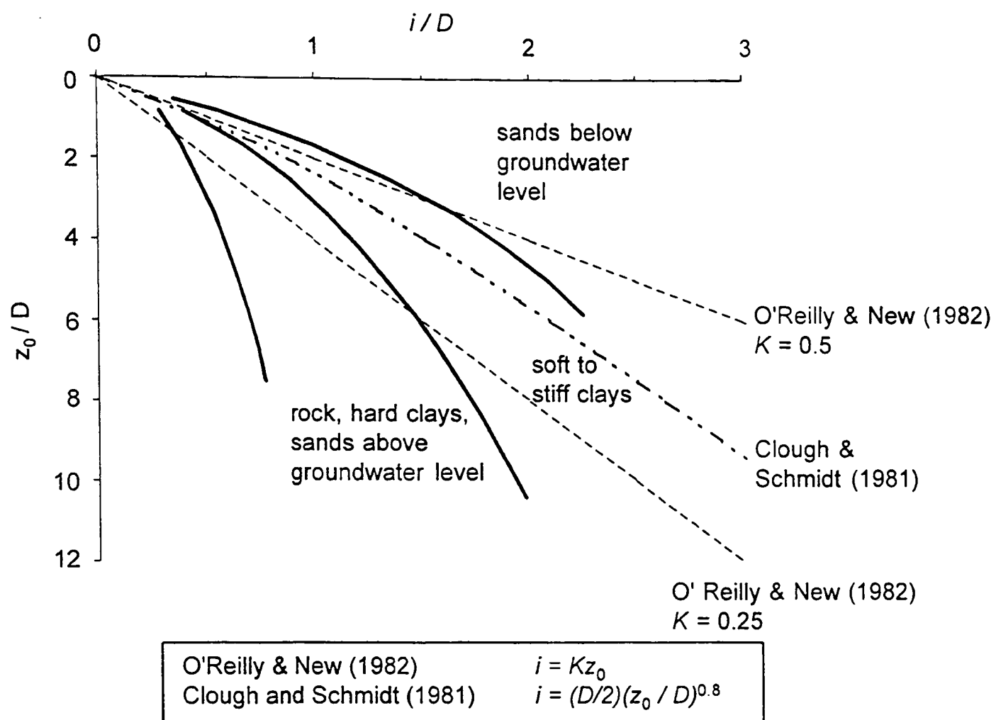
Figure 2.8 Relationships between i at the ground surface and depth of tunnel (originally after Peck, 1969)
