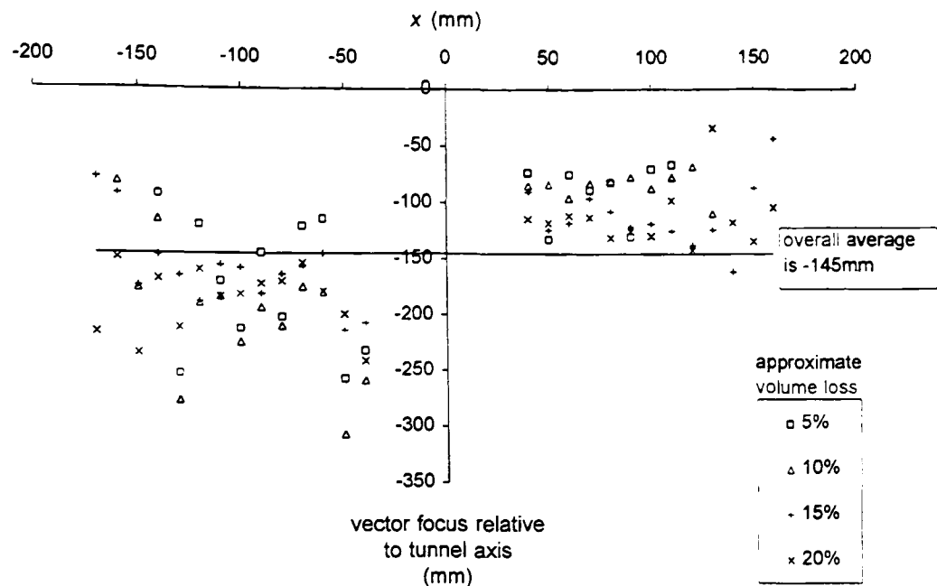
a) 130mm above tunnel axis
