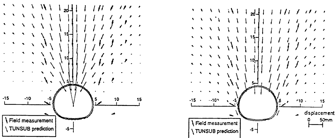
a) Predictions using a point sink at tunnel axis level
