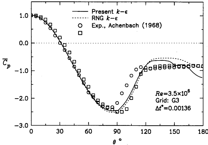
Figure 5.27: Predicted and measured time-averaged wall pressure coefficient for a circular cylinder ( Re = 3.5 \times 10^6 ).
