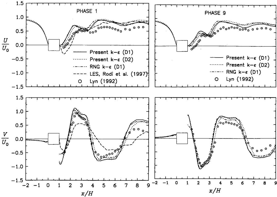
Figure 5.20: Predicted and measured phase-averaged (phases 1, 9) axial (top) and vertical (bottom) velocity profiles along the centreline ( Re = 20000 ).
