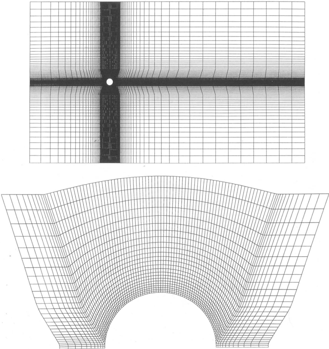
Figure 4.3: Representative numerical grid D1 - 143 \times 98 for a circular cylinder.
