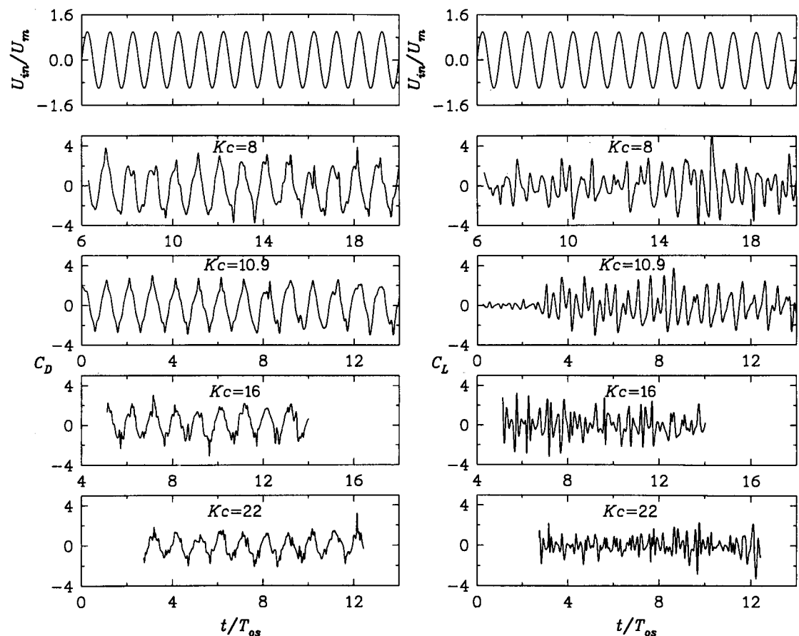
Figure 4.35: Circular cylinder in pure oscillatory flows. Computed drag (left) and lift (right) coefficients versus time at various higher Kc -numbers for \beta = 196 (top curves show the inlet velocity variation).
