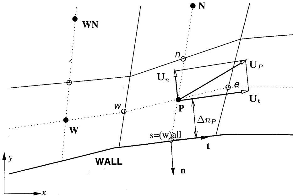
Figure 3.5: Application of the wall boundary conditions.
