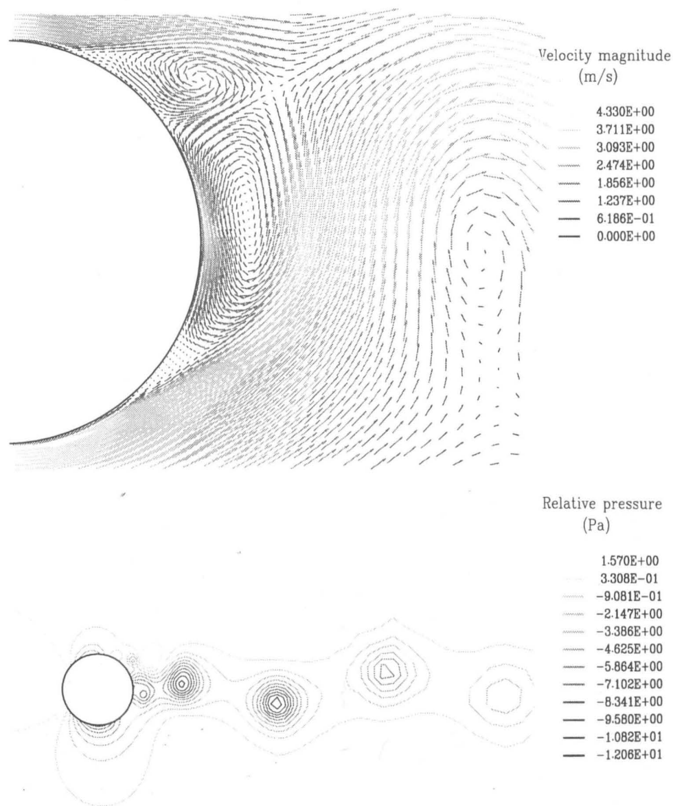
Figure 5.25: Flow past a circular cylinder at Re = 1.4 \times 10^5 . Velocity vectors (top) and pressure contours (bottom) as computed by the unsteady k - \epsilon model at t^* = 117.6 (minimum C_L ).
