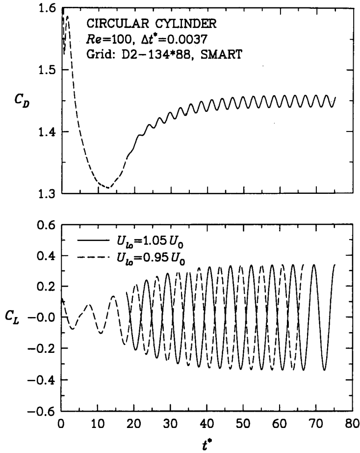
Figure 4.4: Circular cylinder at Re = 100 . Time histories of the drag coefficient (top) and lift coefficient (bottom) as obtained with two initial asymmetric perturbations.
