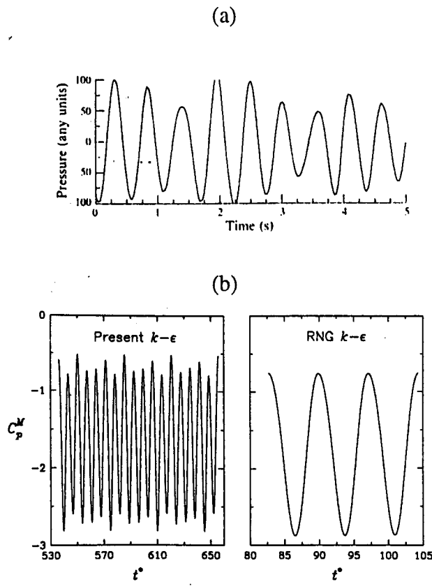
Figure 5.19: Time traces of the pressure signal monitored at the middle of the top face: (a) measurements of Lyn (1992), (b) present computations.
