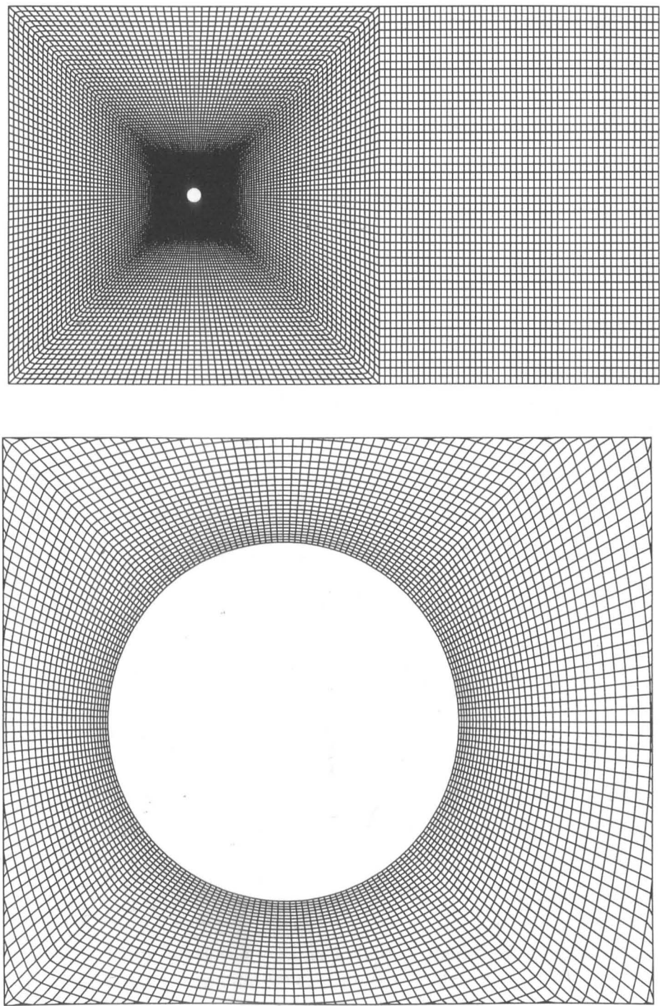
Figure 5.23: Numerical grid G1 used for the flow past a circular cylinder at Re = 1.4 \times 10^5 .
