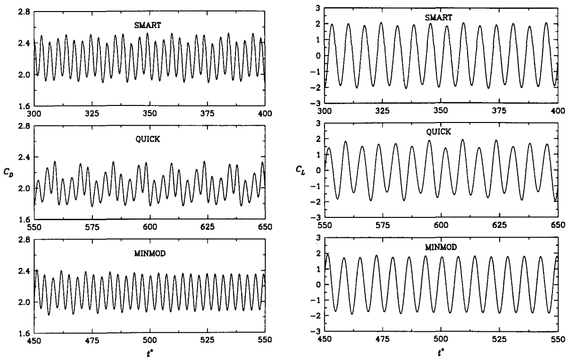
Figure 5.9: Turbulent flow around a square cylinder at Re = 20000 . Time traces of the drag (left) and lift (right) coefficients as calculated by three convective schemes.
