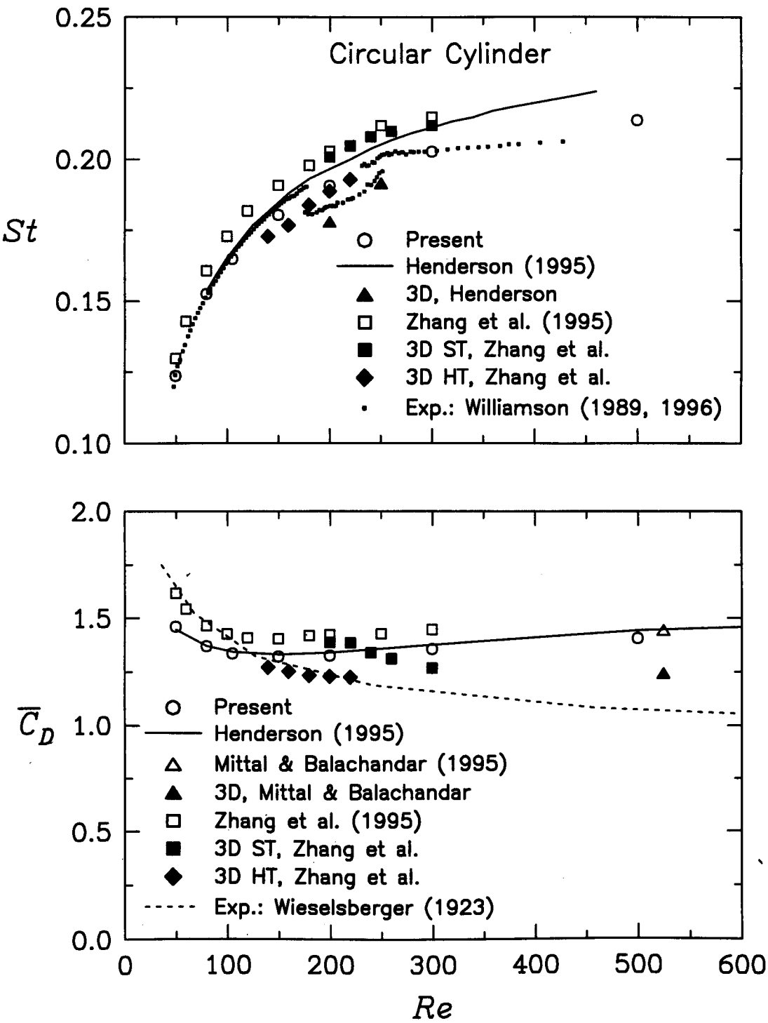
Figure 4.30: Flow past a circular cylinder. Comparisons between 2-D and 3-D simulations and experiments (present predictions with the grid D1 - 143 \times 98 and SMART scheme).
