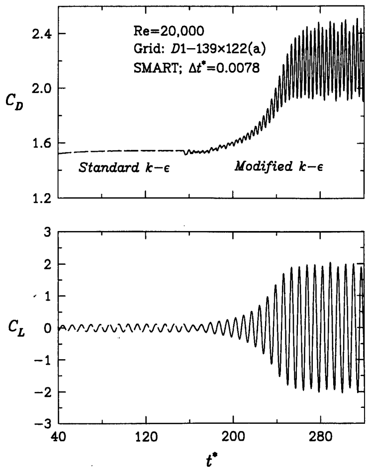
Figure 5.5: Turbulent flow past a square cylinder at Re = 20,000 . Time evolution of the drag (top) and lift (bottom) coefficients as predicted by the k - \epsilon model before and after the unsteady modification.
