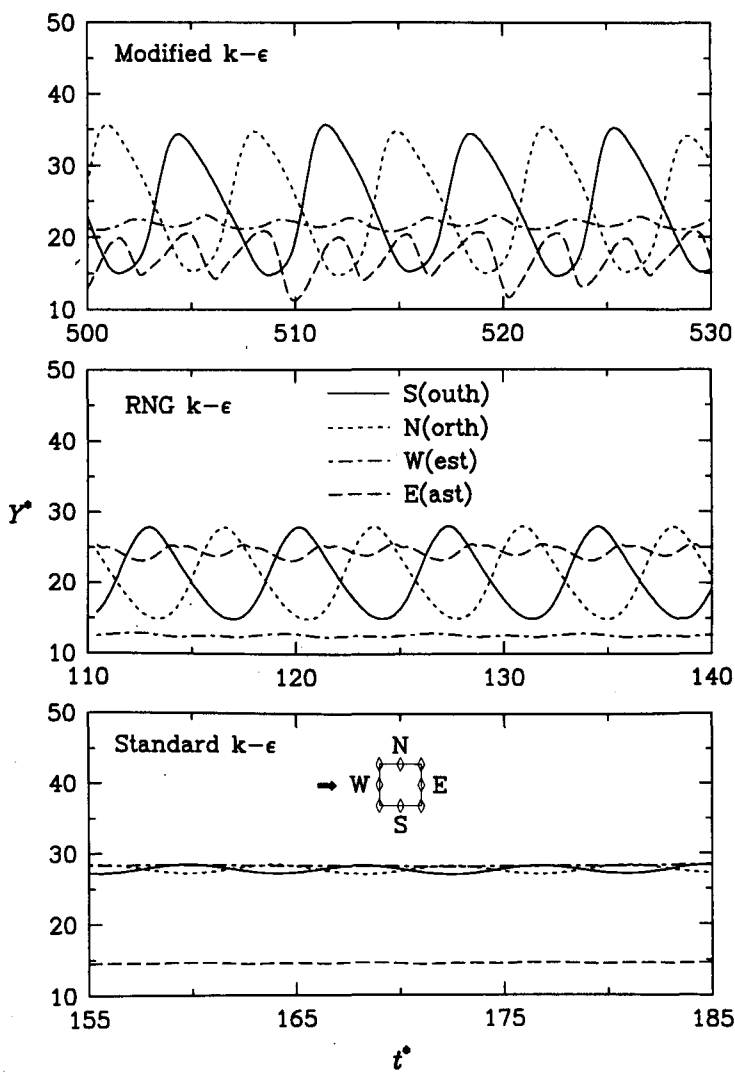
Figure 5.7: Wall units Y^* versus time as predicted by the k - \epsilon models ( Re = 20000 ).
