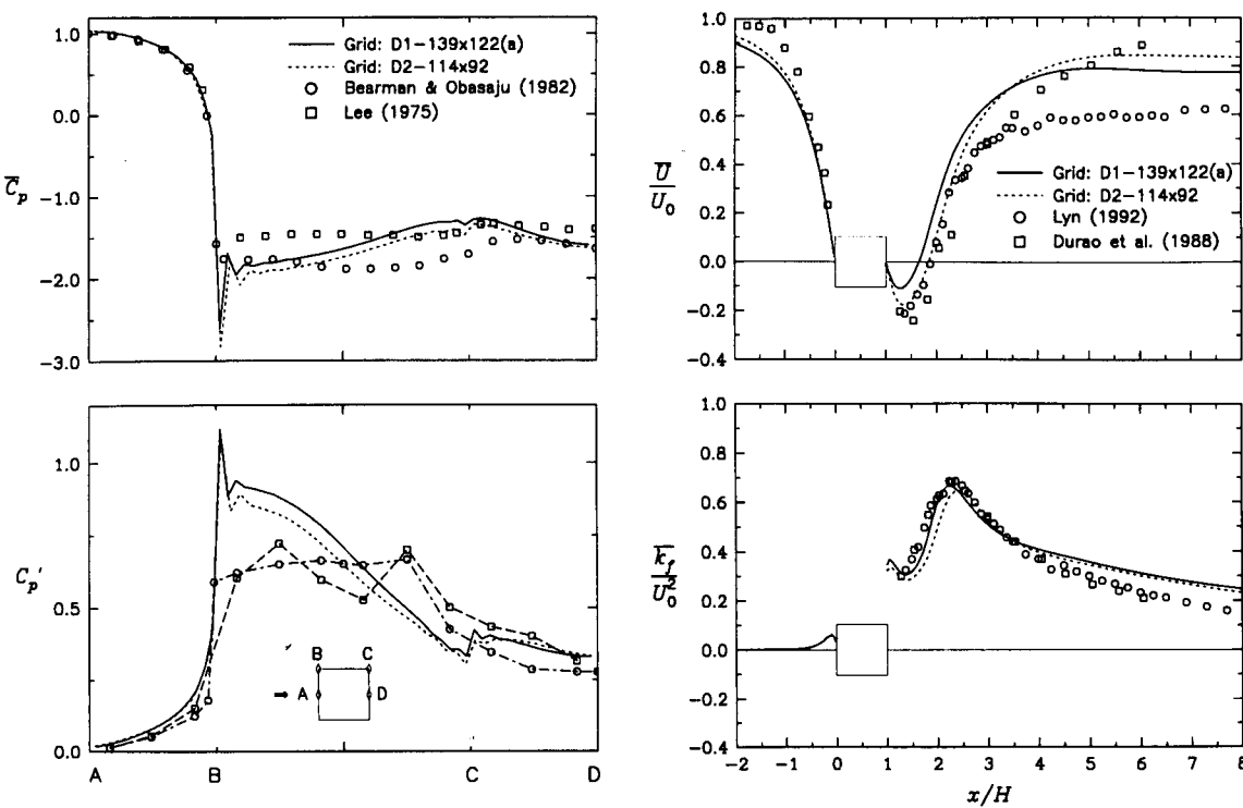
Figure 5.13: Domain size influence on the distributions of time-averaged flow quantities: (left) the pressure coefficients, (right) the streamwise velocity and fluctuating kinetic energy.
