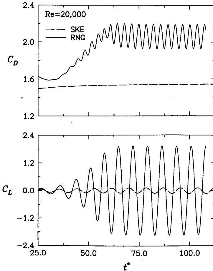
Figure 5.3: Turbulent flow past a square cylinder at Re = 20,000 . Time evolution of the drag (top) and lift (bottom) coefficients as predicted by the standard and RNG k - \epsilon models (grid D1 - 139 \times 122(a) , SMART scheme).
