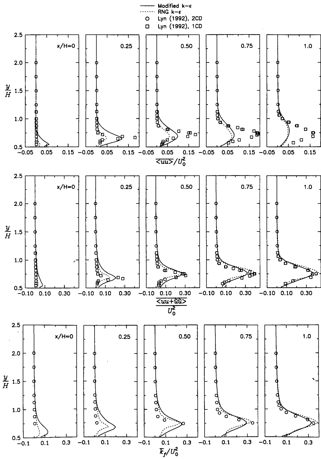
Figure 5.18: The time-averaged profiles of the Reynolds stress component \langle \overline{u^2} \rangle (top), apparent component \langle \overline{u^2 + \tilde{u}^2} \rangle (middle) and global fluctuating kinetic energy k_f (bottom) at several lateral cross-sections along the upper side of a square cylinder.
