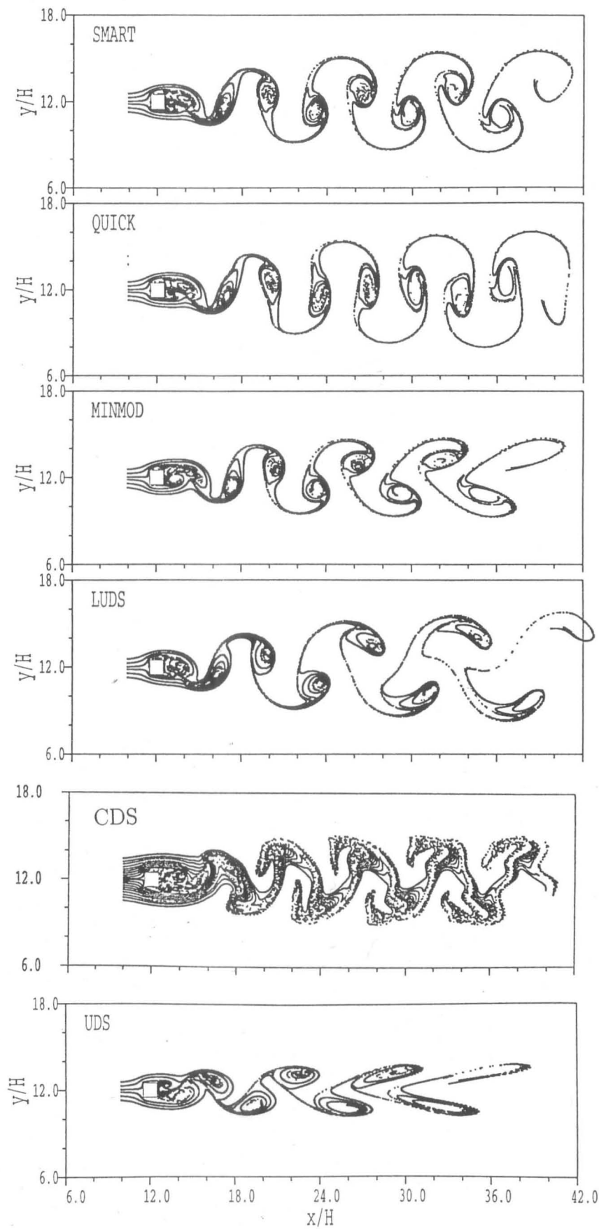
Figure 4.17: Flow past a square cylinder at Re = 250 . Streaklines computed with different convective schemes.
