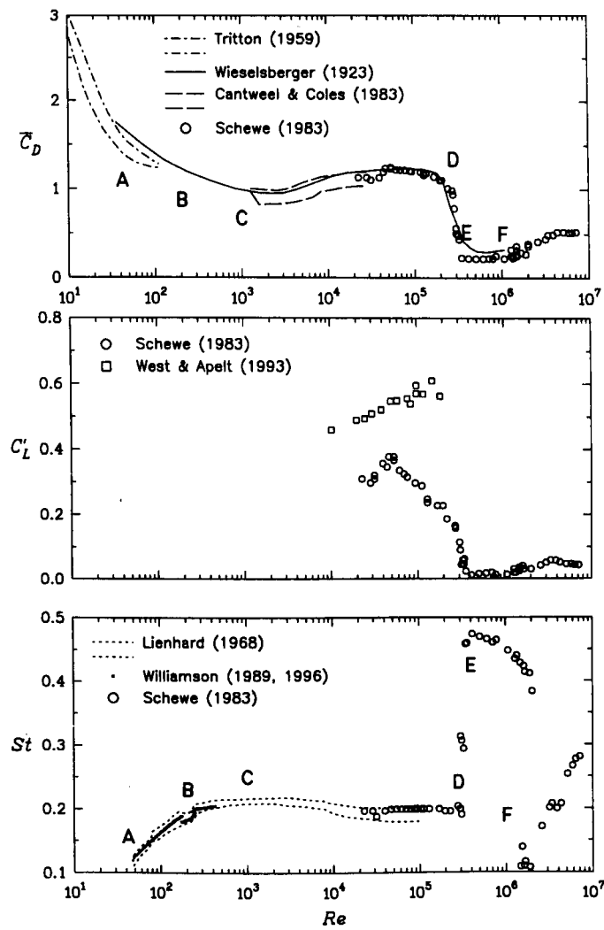
Figure 1.2: Vortex shedding parameters vs. Re for a smooth circular cylinder in a uniform low-turbulence stream: the mean drag coefficient (top), r.m.s. lift coefficient (middle) and Strouhal number (bottom).
