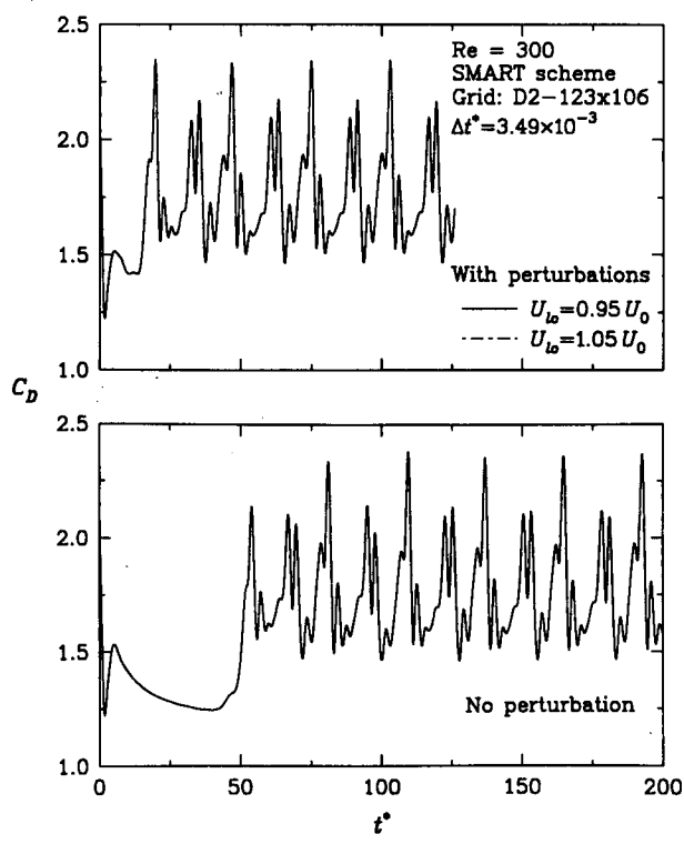
Figure 4.25: Flow around a square cylinder at Re = 300 . Time traces of the drag coefficient as calculated with two initial perturbations (top) and without it (below).
