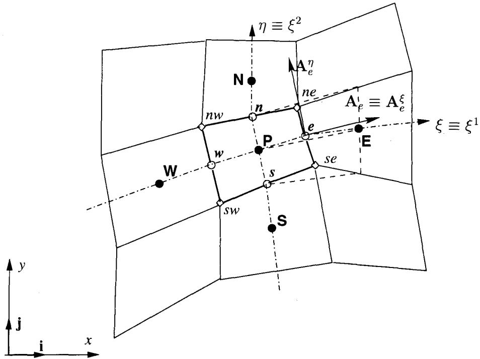
Figure 3.1: A typical control volume and the points-of-compass notation used for the cell-centred two-dimensional structured grid ( \bullet , locations of variables solved for; \circ , locations where fluxes are required).
