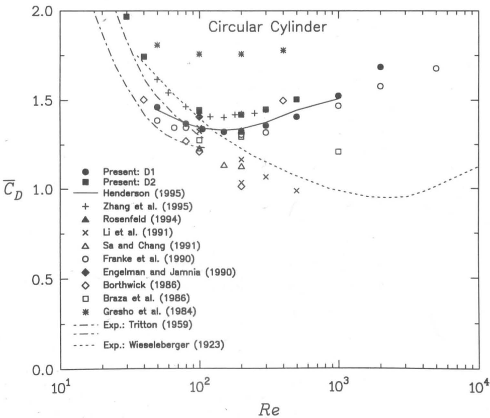
Figure 4.29: Flow past a circular cylinder. Comparison of the computed mean drag coefficients (the grids D1-143x98 and D2-134x88; SMART scheme) with others.
