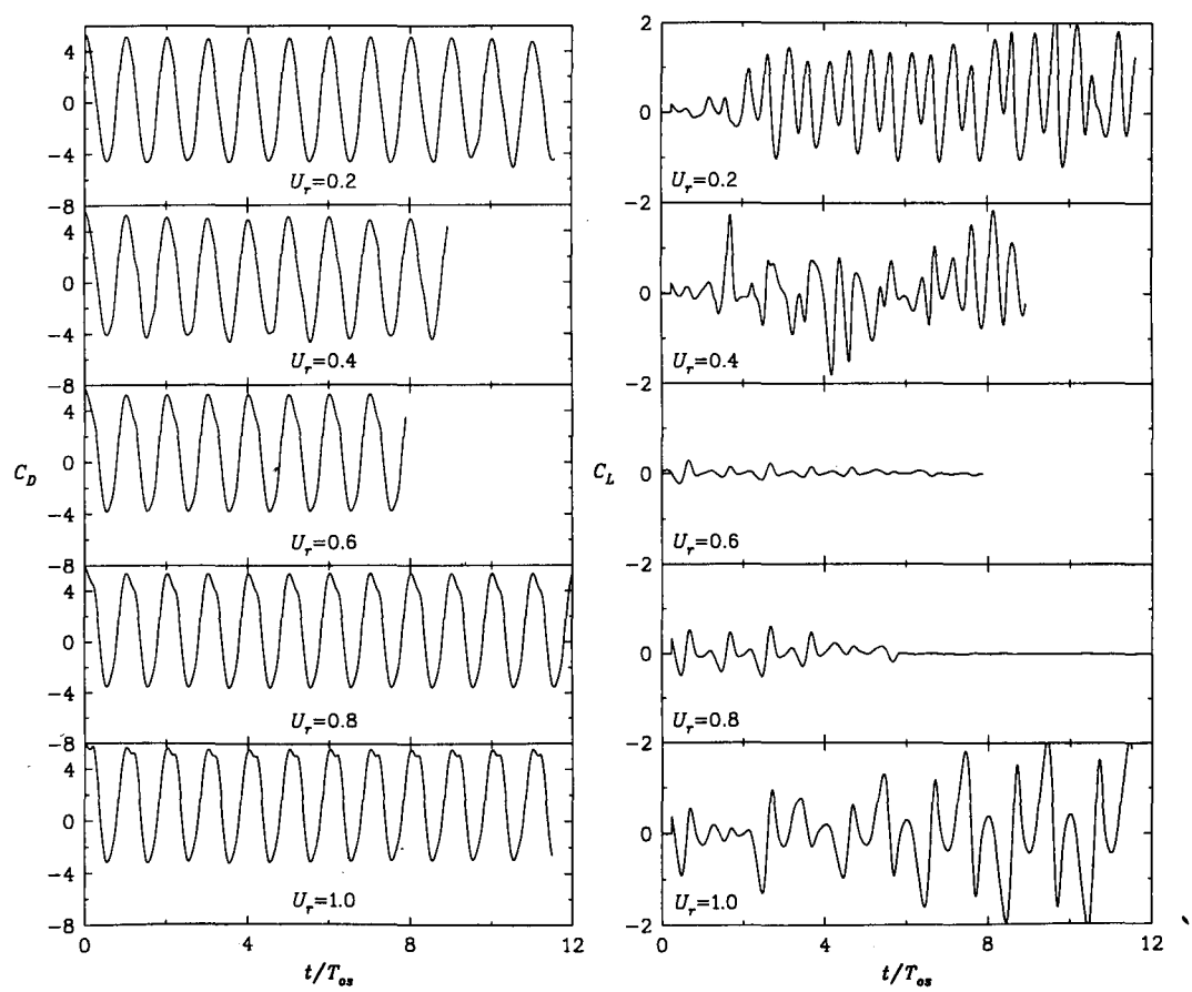
Figure 4.37: Circular cylinder in current plus oscillations. Time histories of the drag (left) and lift (right) coefficients as a function of velocity ratio.
