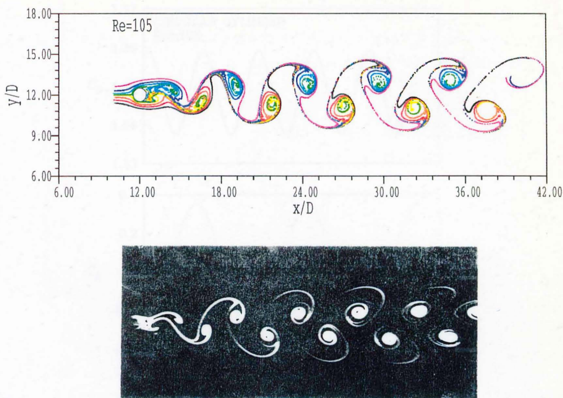
Figure 4.12: Streaklines for a circular cylinder at Re = 105 : (a) computed at t^* = 204.9 (where the lift coefficient is at maximum); (b) photograph from experiments by S. Taneda, van Dyke (1982).
