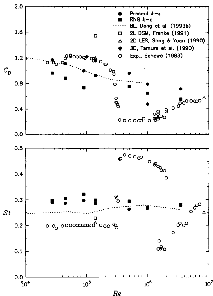
Figure 5.28: Turbulent flow around a circular cylinder. Comparison of the computed mean drag coefficient (top) and the Strouhal number (bottom) with others.
