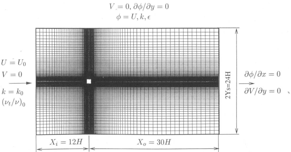
Figure 5.1: Numerical grid D1 - 139 \times 122(a) and boundary conditions for the flow around a square cylinder.
