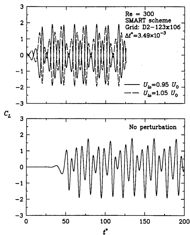
Figure 4.24: Flow around a square cylinder at Re = 300 . Time traces of the lift coefficient as calculated with two initial perturbations (top) and without it (below).
