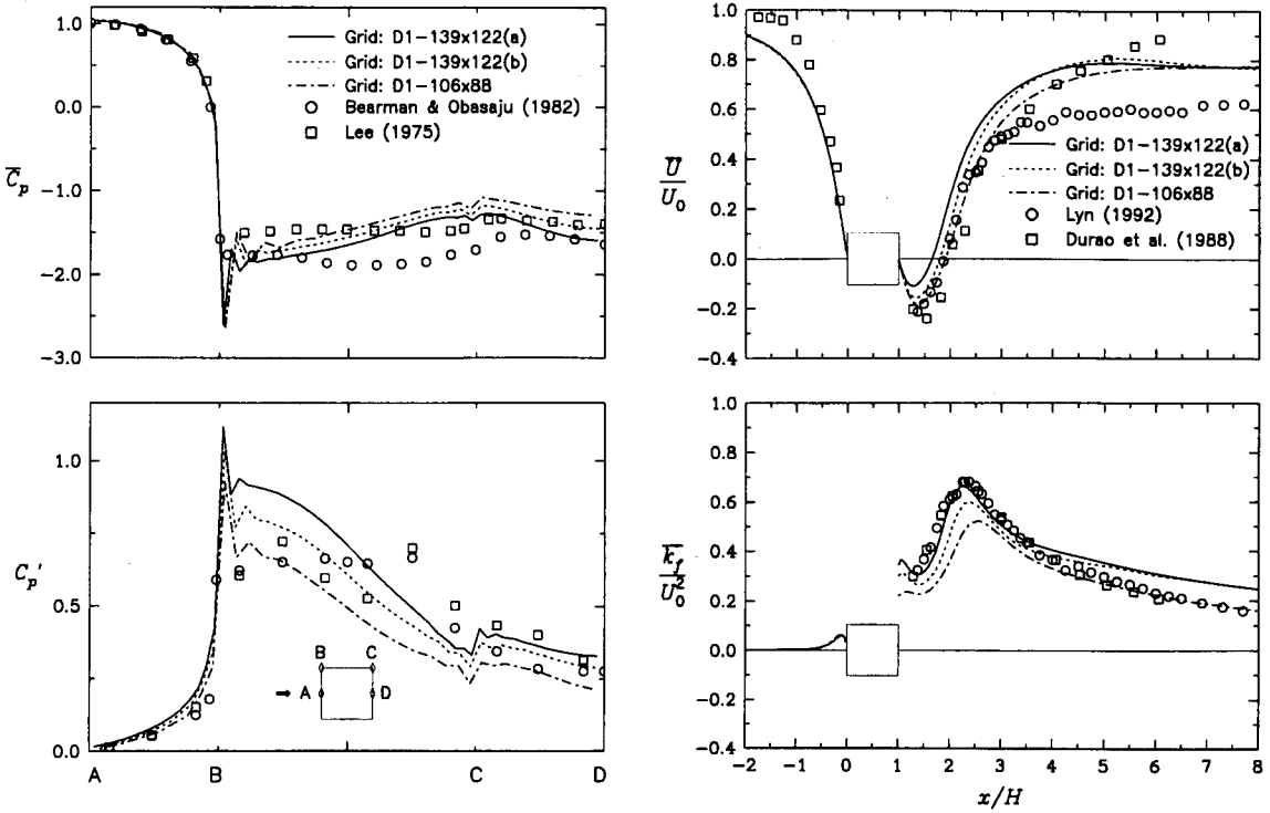
Figure 5.12: Grid resolution effects on the distribution of time-averaged flow quantities: (left) the pressure coefficients, (right) the streamwise velocity and fluctuating kinetic energy.
