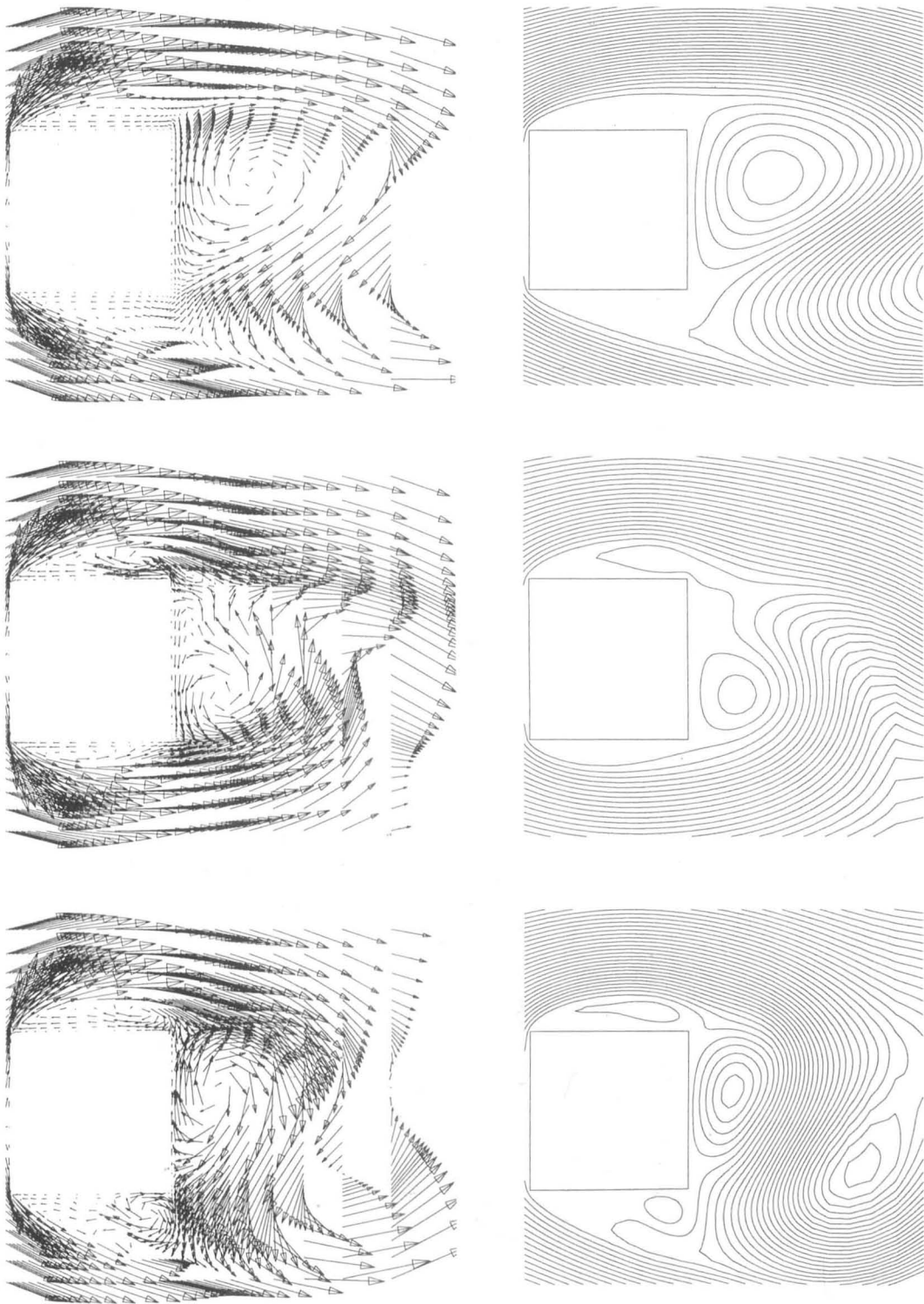
Figure 4.23: Velocity vectors and streamlines around a square cylinder showing the flow reattachment at the cylinder sides: (top) Re = 300 , (middle) Re = 500 , and (bottom) Re = 1000 (grid D1-136x118, SMART scheme).
