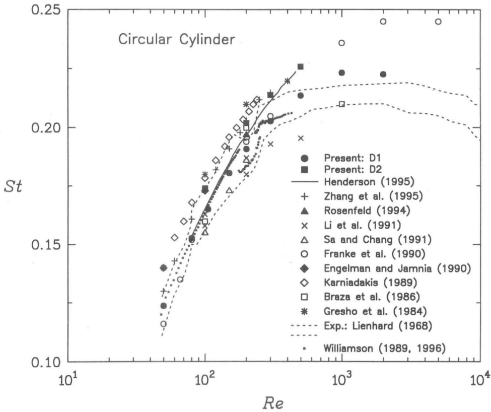
Figure 4.28: Flow past a circular cylinder. Comparison of the computed Strouhal numbers (the grids D1-143x98 and D2-134x88; SMART scheme) with others.
