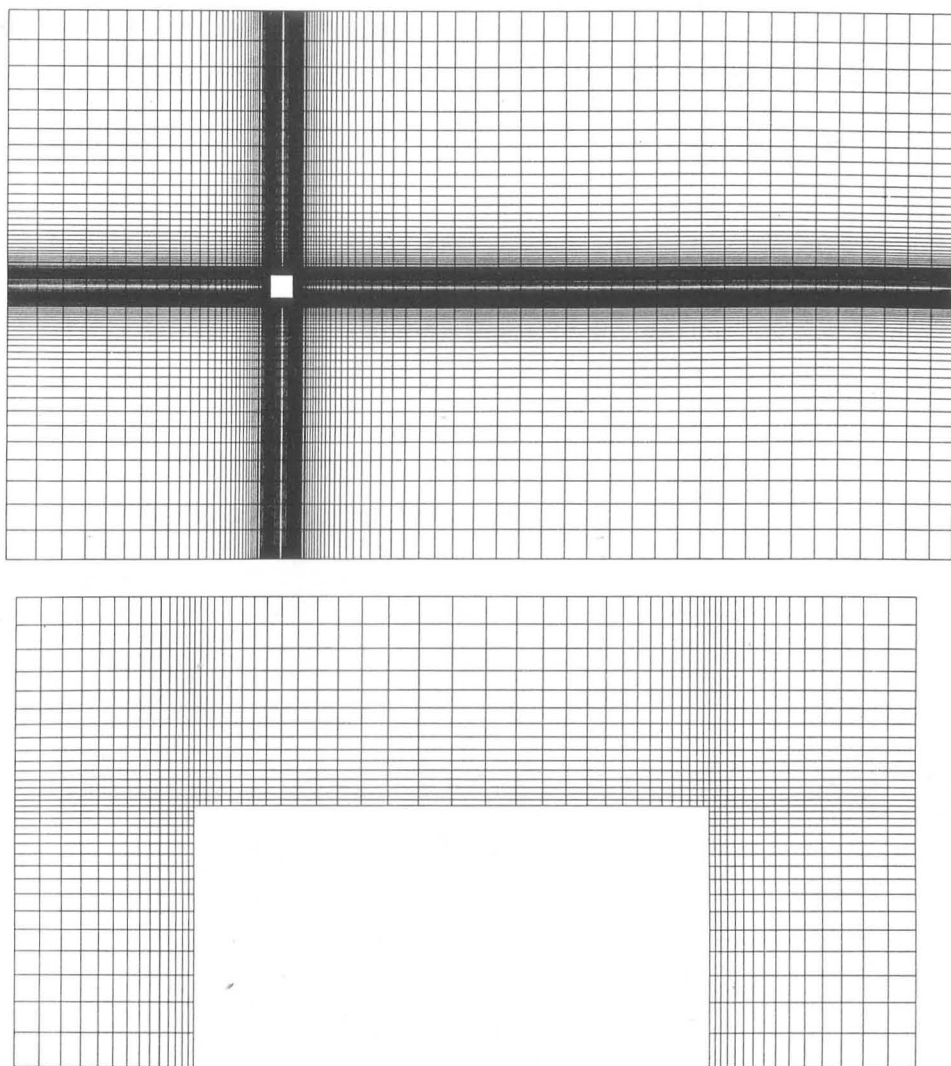
Figure 4.2: Representative numerical grid of D1 - 136 \times 118 for a square cylinder.
