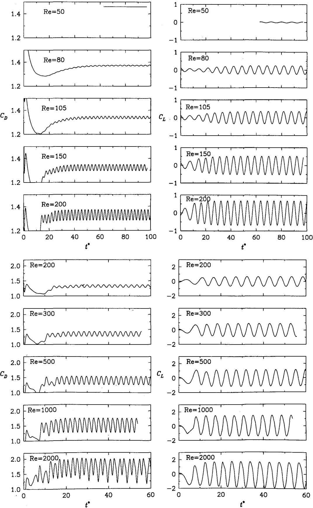
Figure 4.27: Time history of the drag coefficient (left) and the lift coefficient (right) for vortex shedding from a circular cylinder as a function of Reynolds numbers (grid D1-143x98, SMART scheme).
