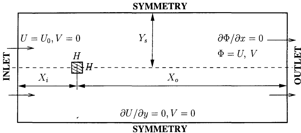
Figure 4.1: Typical solution domain and boundary conditions.
