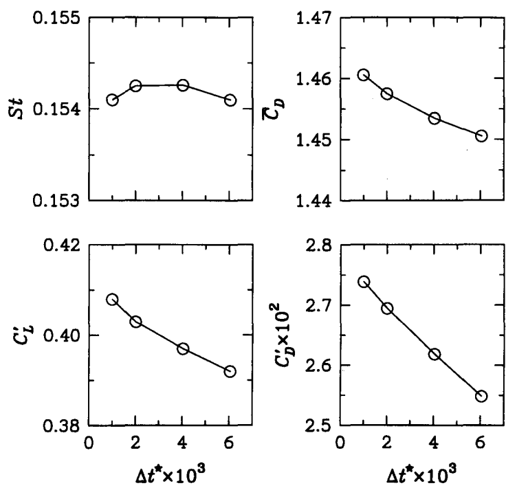
Figure 4.15: Flow past a square cylinder at Re = 200 . Effect of the time step size on the vortex shedding parameters (grid D1-136x118, SMART scheme).
