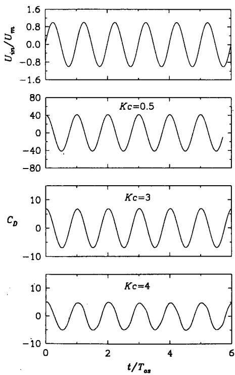
Figure 4.34: Circular cylinder in pure oscillatory flows. Computed drag coefficients versus time at Kc = 0.5, 3 , and 4 and \beta = 196 (the top curve shows the inlet velocity variation).
