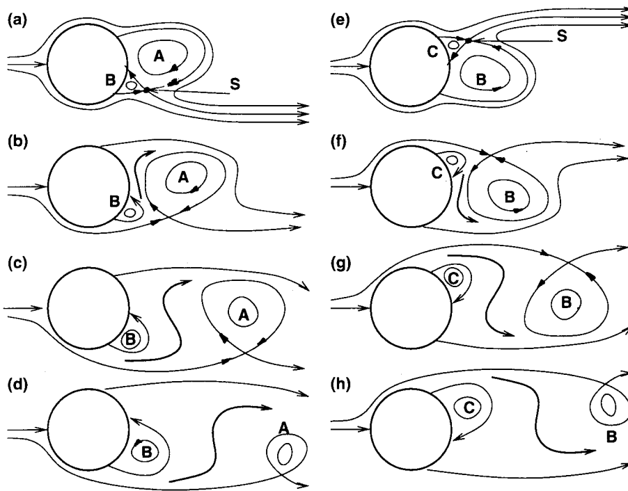
Figure 4.10: Model of periodic vortex shedding using topology of instantaneous streamlines (separatrices).
