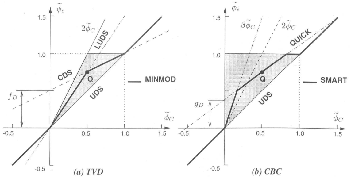
Figure 3.4: Graphical representation of TVD (left) and CBC (right) criteria and NVD characteristics of some bounded schemes.
