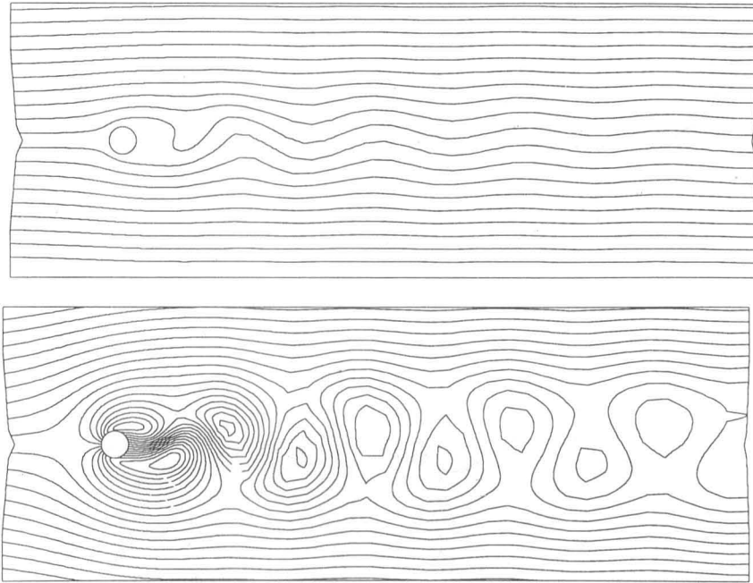
Figure 4.11: Karman vortex street for a circular cylinder at Re = 105 . Streamlines using fixed frame of reference (top) and with frame of reference in translation at velocity 0.85 U_0 (bottom).
