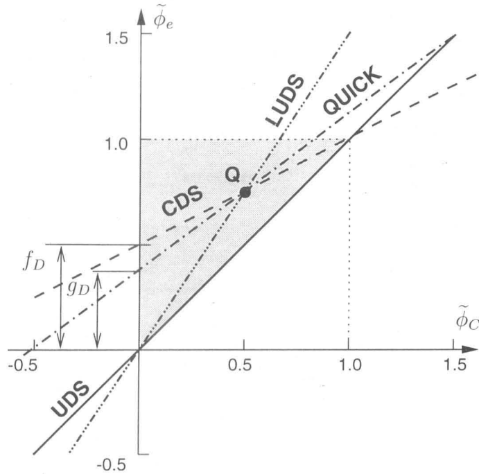
Figure 3.3: NVD diagram for several convective schemes.
