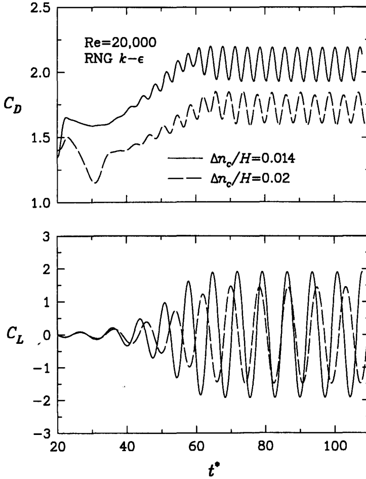
Figure 5.4: Turbulent flow past a square cylinder at Re = 20,000 . Time evolution of the drag (top) and lift (bottom) coefficients as predicted by RNG k - \epsilon model with two near-wall cell distances (grids D1 - 139 \times 122(a, b) , SMART scheme).
