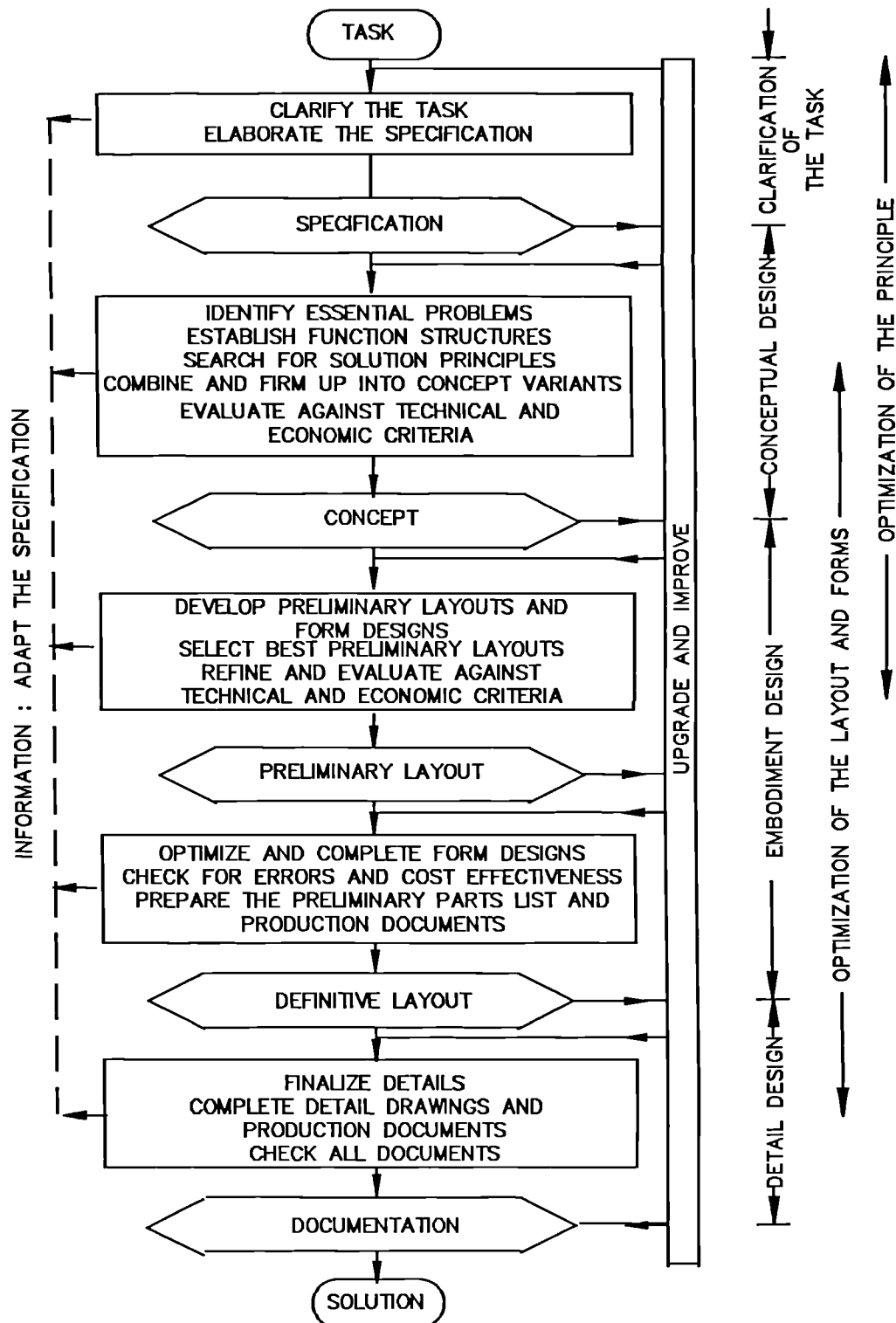
Figure 2.10 The Design Model by Pahl & Beitz
