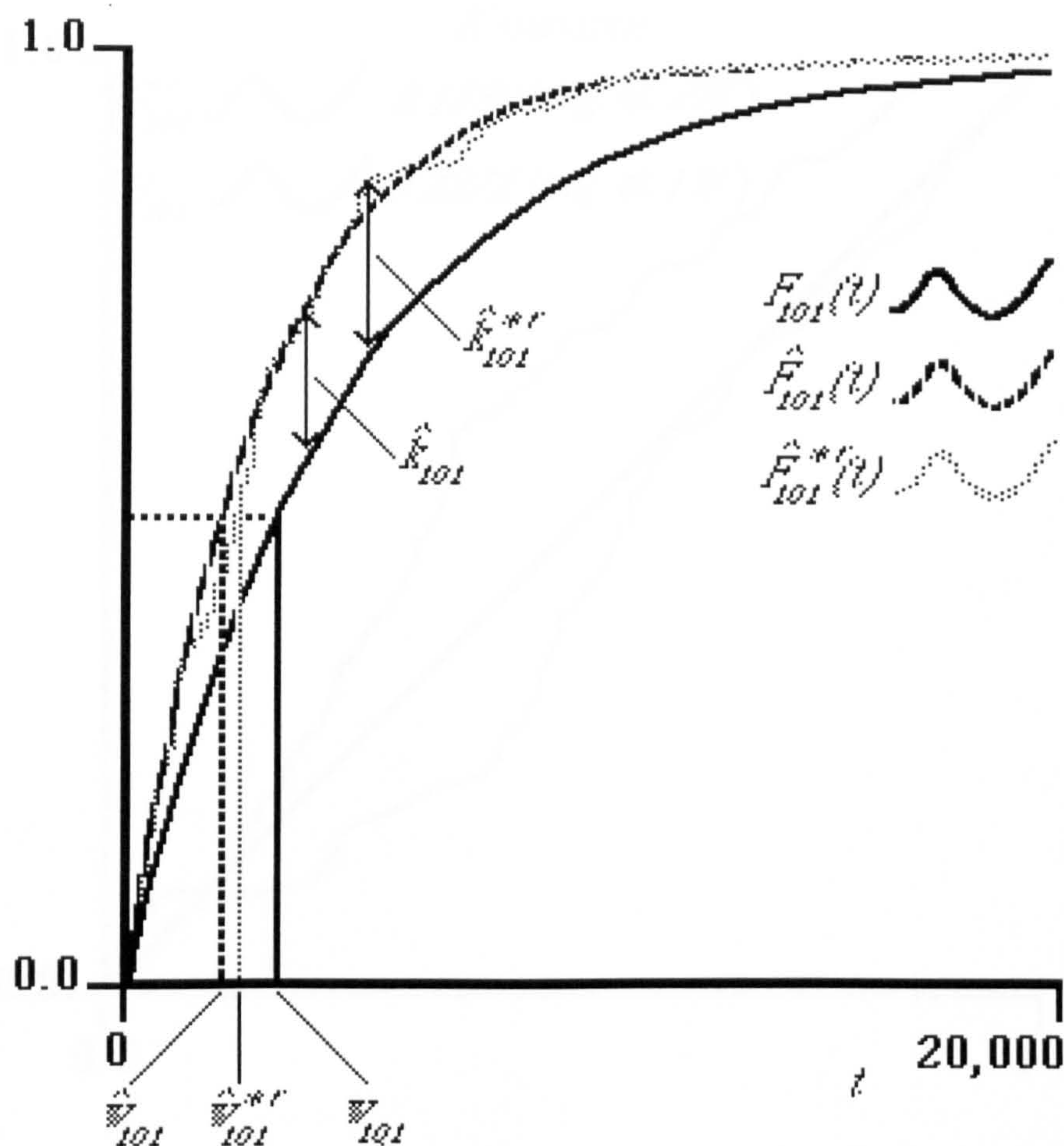
Figure 4.1-2. True, raw and retrodictive recalibrated cdfs of T_{101} for the DU model and data set 7 generated by the L model.
