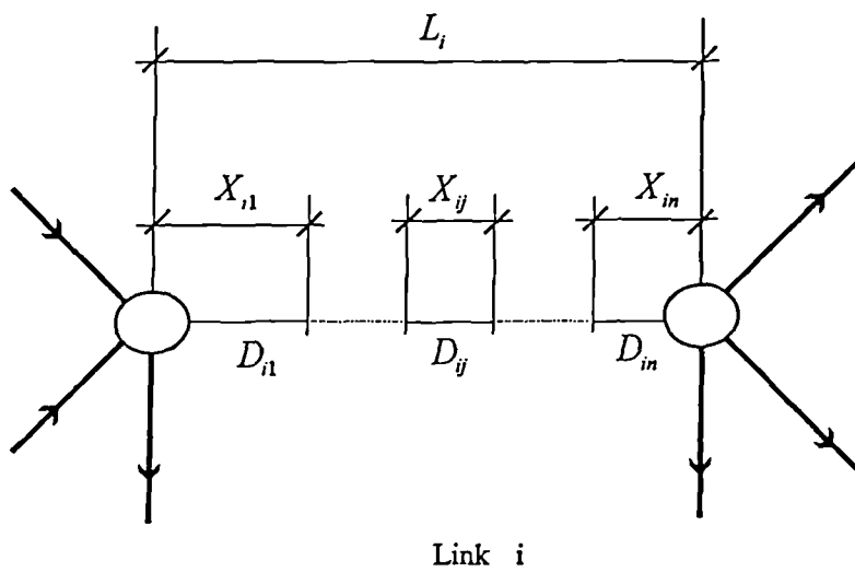
Figure 6.2 Representation of Segment X_{ij} in a Link of Length L_i
