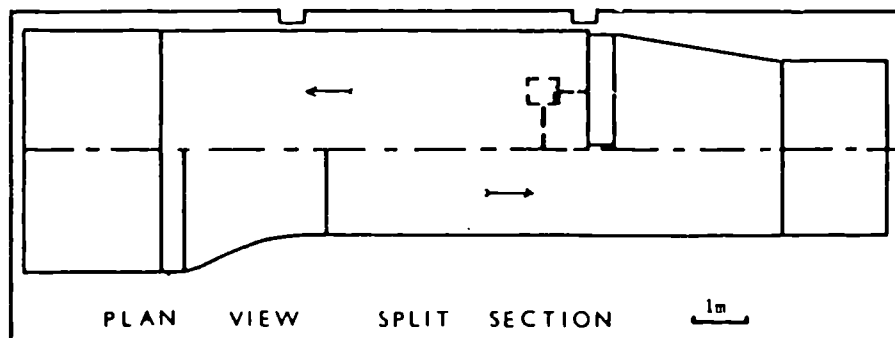
Wind tunnel layout.
