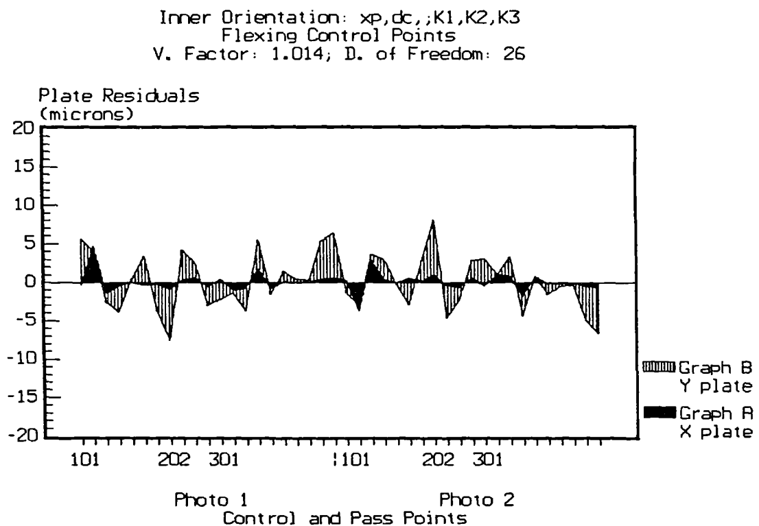
Figure 5.9 Photo-coordinate residuals- BINFLEXPC
