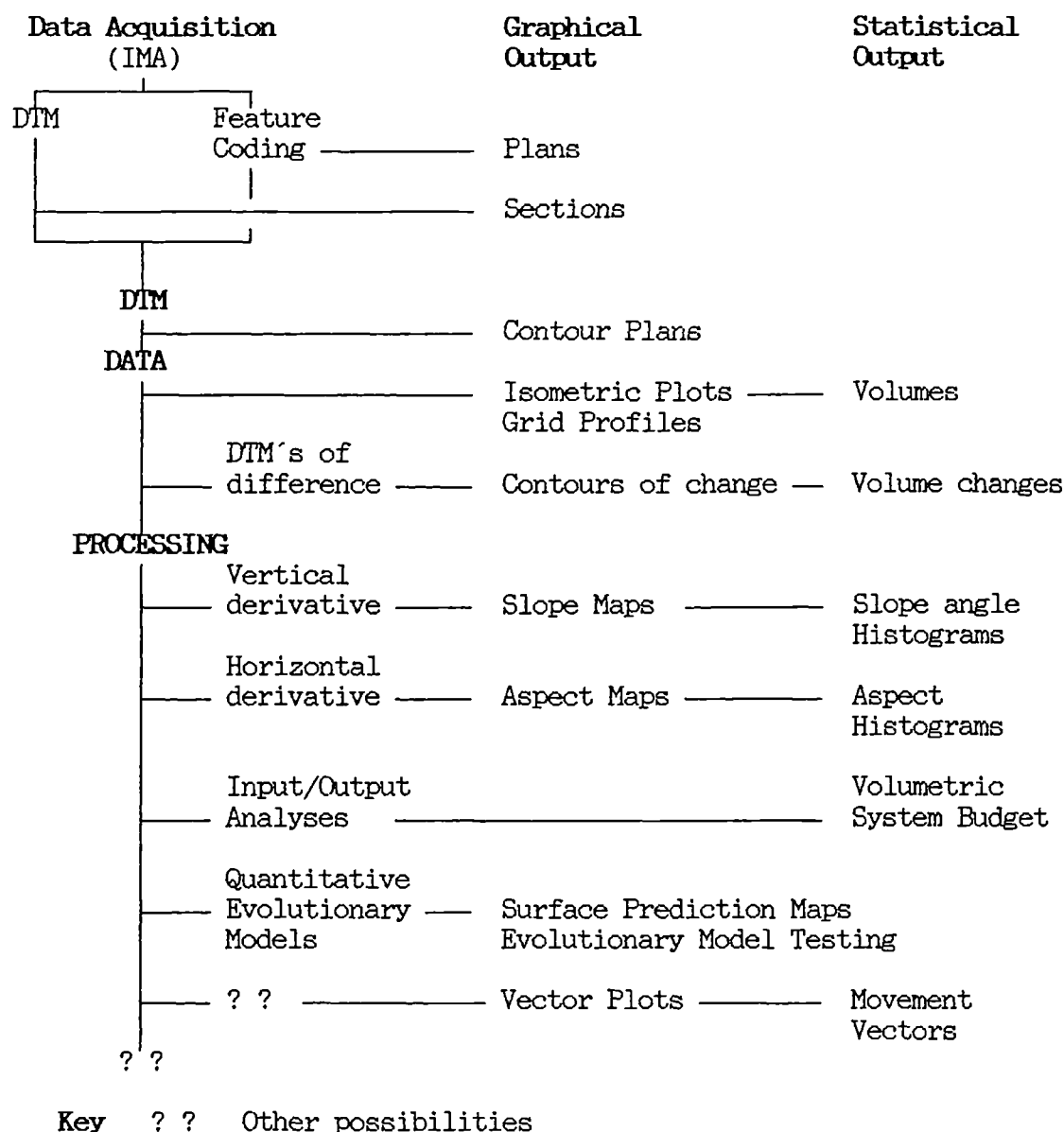
Figure 7.1 Geomorphic Data Processing
