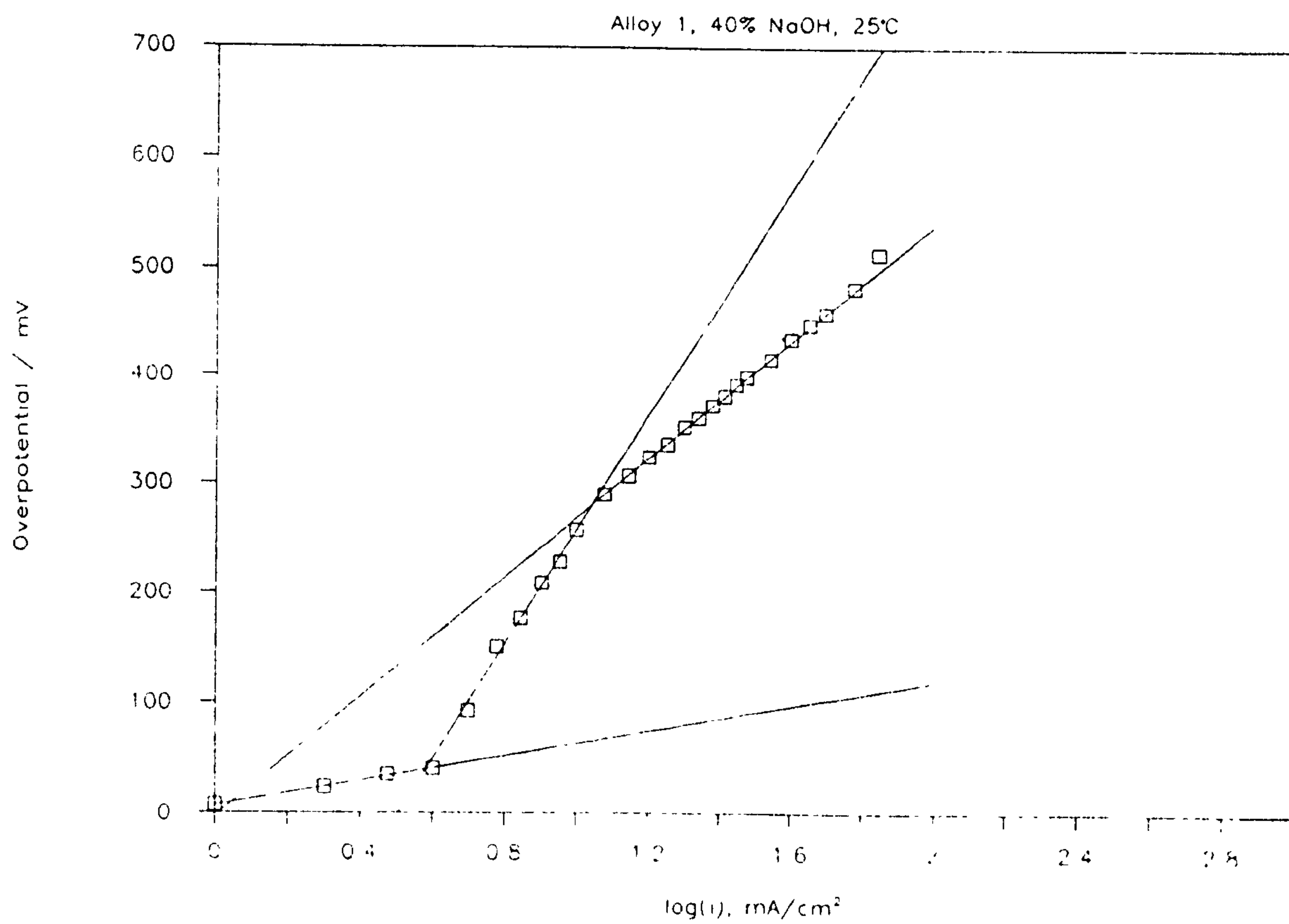
Figure 4.18 Tafel Plots
