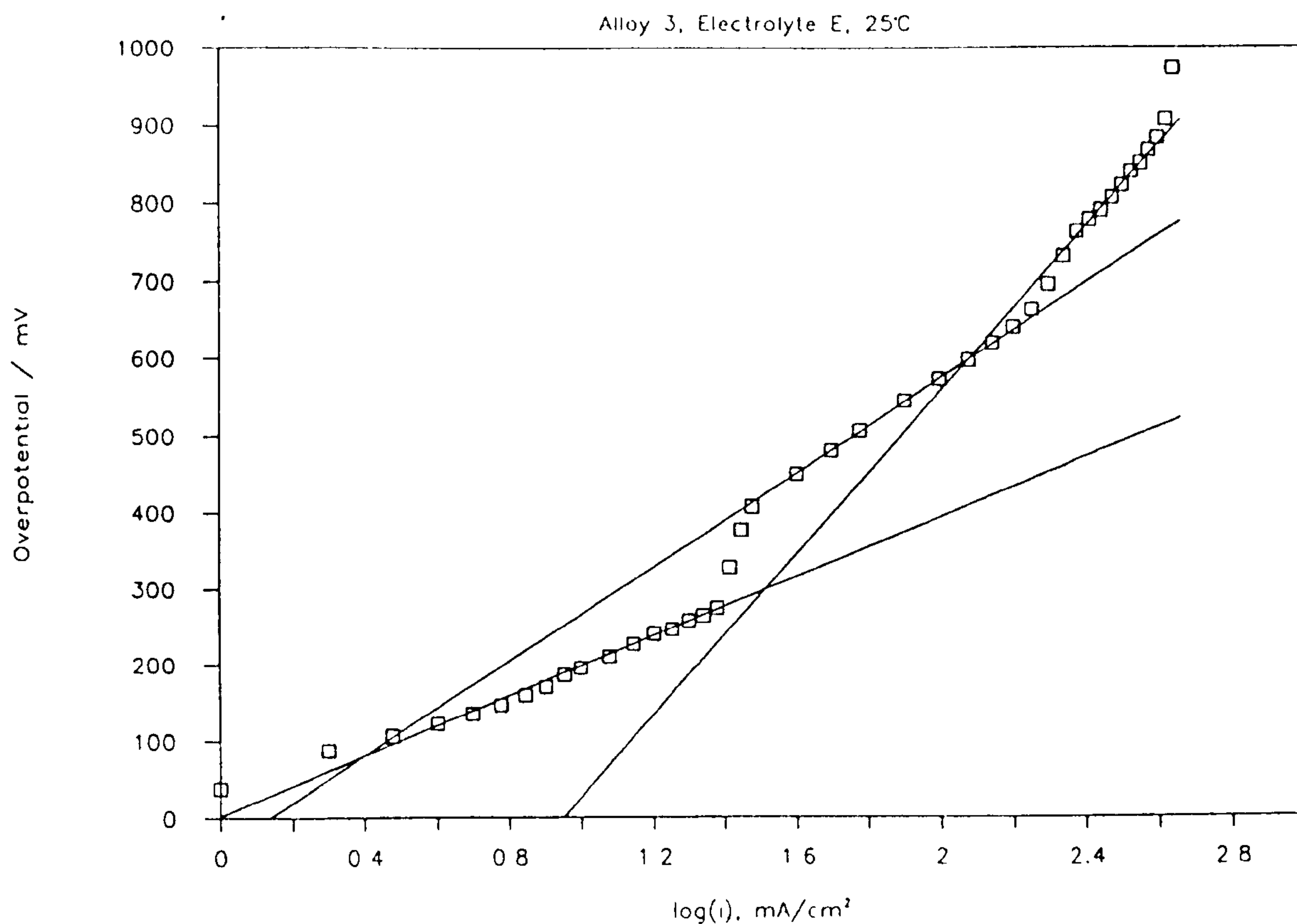
Figure 4.15 Tafel Plots
