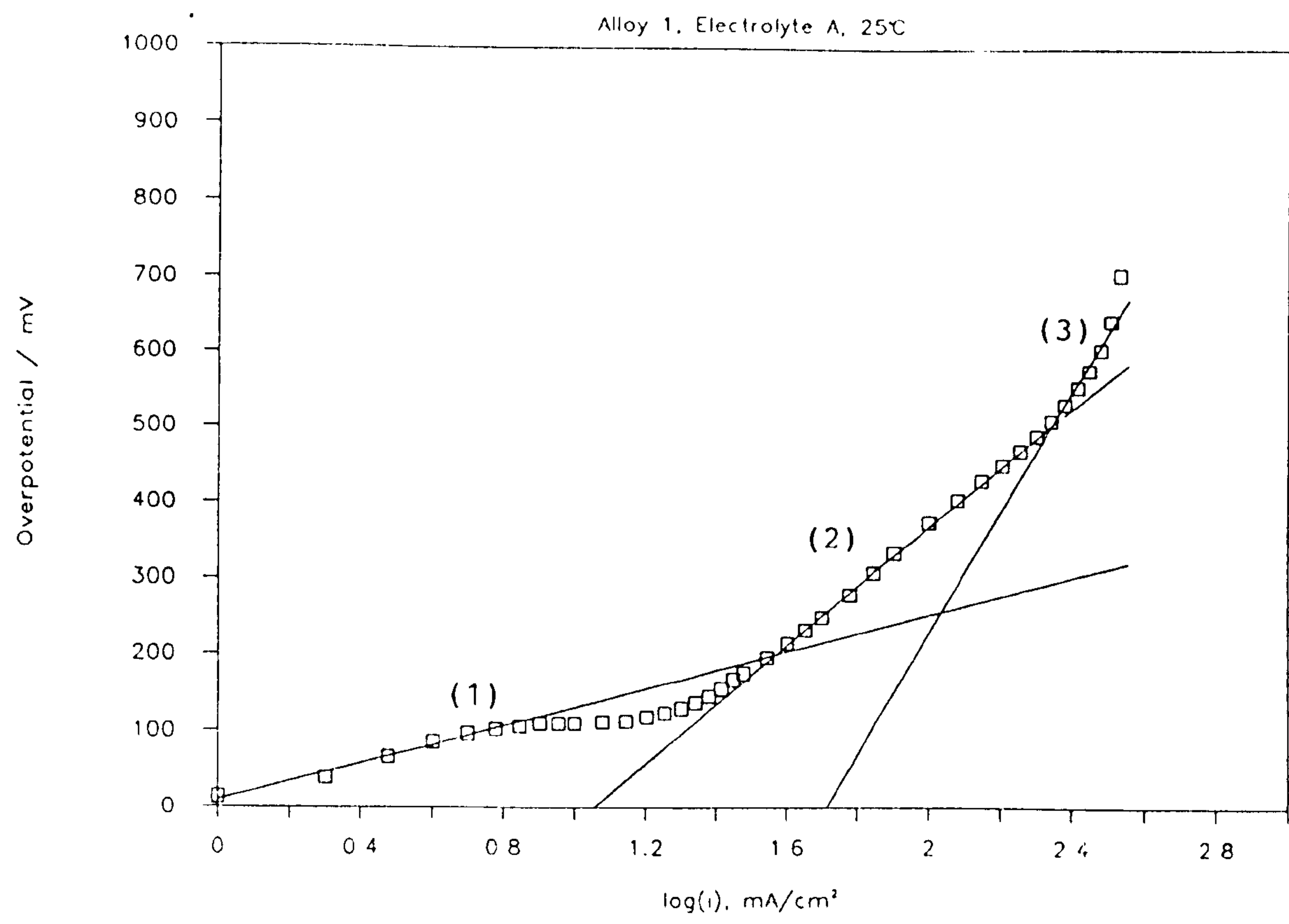
Figure 4.8 Tafel Plots
