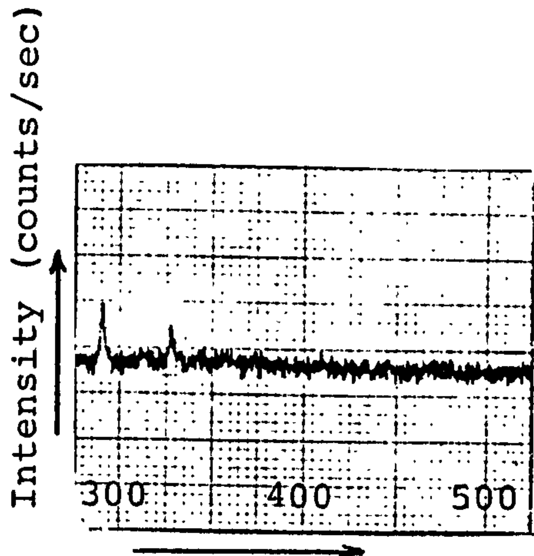
Alloy 2, before discharge, after Argon etching. No evidence of tin or titanium.
