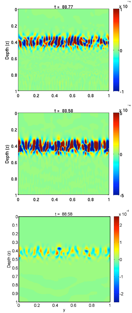
Figure 2. A comparison of the vertical component of velocity at comparable times for a slice of the three-dimensional case (top) and a quasi-two-dimensional run (middle). The bottom image shows density perturbation from the horizontal averaged value.
