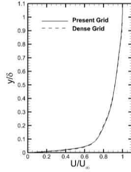
Fig. 4 The boundary layer profiles from different grid resolutions.
