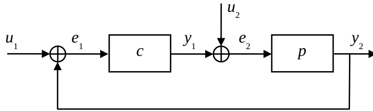
Fig. 2.1: The unity feedback configuration
