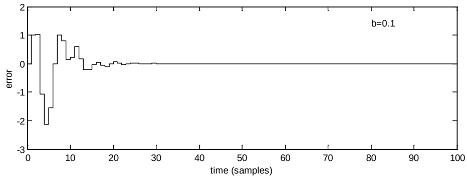
Fig.4.3: Error responses of the disturbed system with \nu = \partial(t^*) = 6
