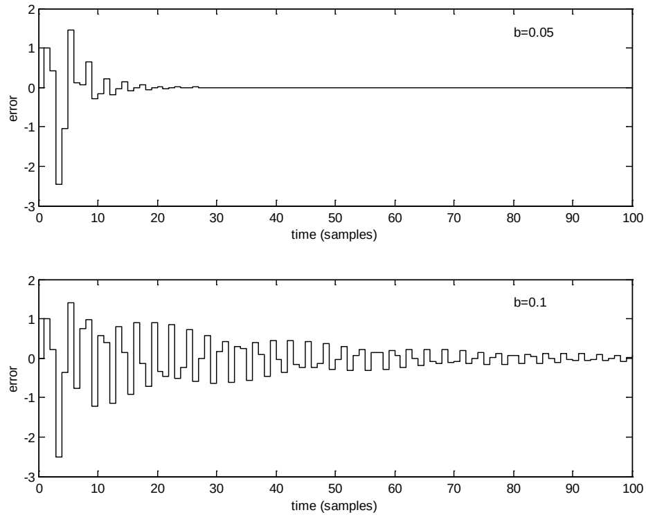
Fig. 4.2: Error responses of the disturbed system with \nu = \partial(t^*) = 3
