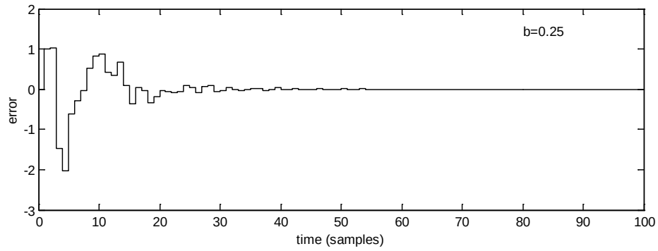
Fig. 4.4: Error responses of the disturbed system with \nu = \partial(t^*) = 9
