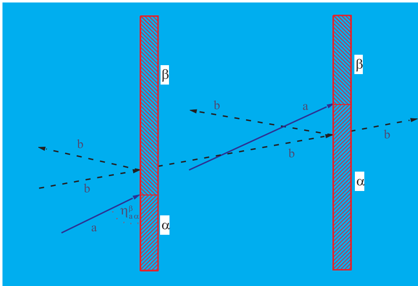
Figure 3: Defect bound state bootstrap equations.
