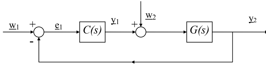
Figure (2.1): Feedback Configuration
