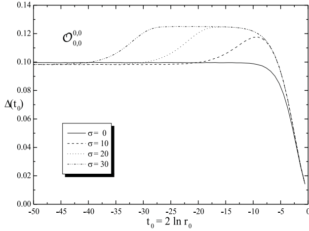
Figure 2: Renormalization group flow for the conformal dimension \Delta(r_0) of the operator \mathcal{O}_{0,0}^{0,0} for various values of the resonance parameter \sigma .
