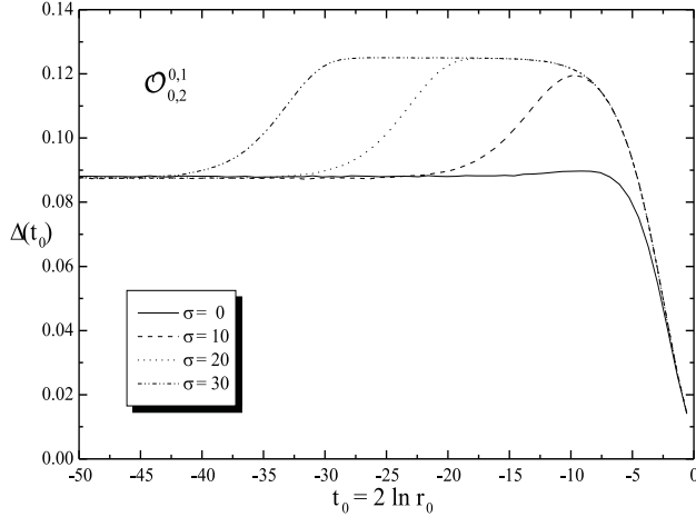
Figure 3: Renormalization group flow for the conformal dimension \Delta(r_0) of the operator \mathcal{O}_{0,2}^{0,1} for various values of the resonance parameter \sigma .
