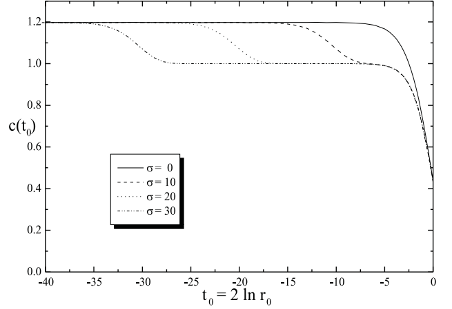
Figure 1: Renormalization group flow for the Virasoro central charge c(r_0) for various values of the resonance parameter \sigma .
