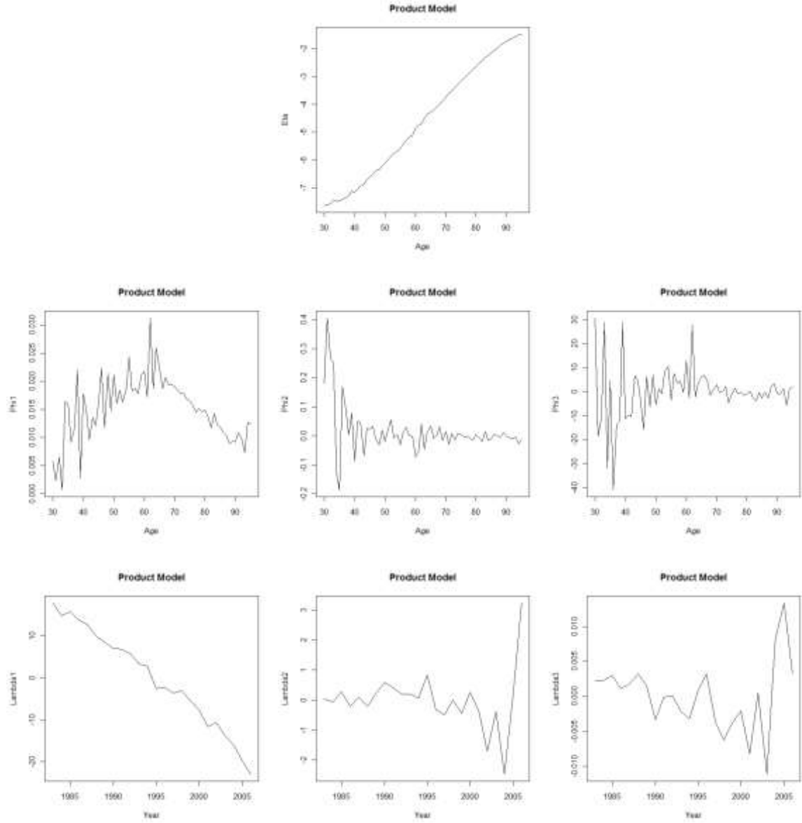
Fig. 4. Parameter estimates of \eta_x (top), \phi_x(j) (middle), and \lambda_t(j) (bottom) of product model of PRM for j = 1, 2, 3 (left to right of last two rows).
