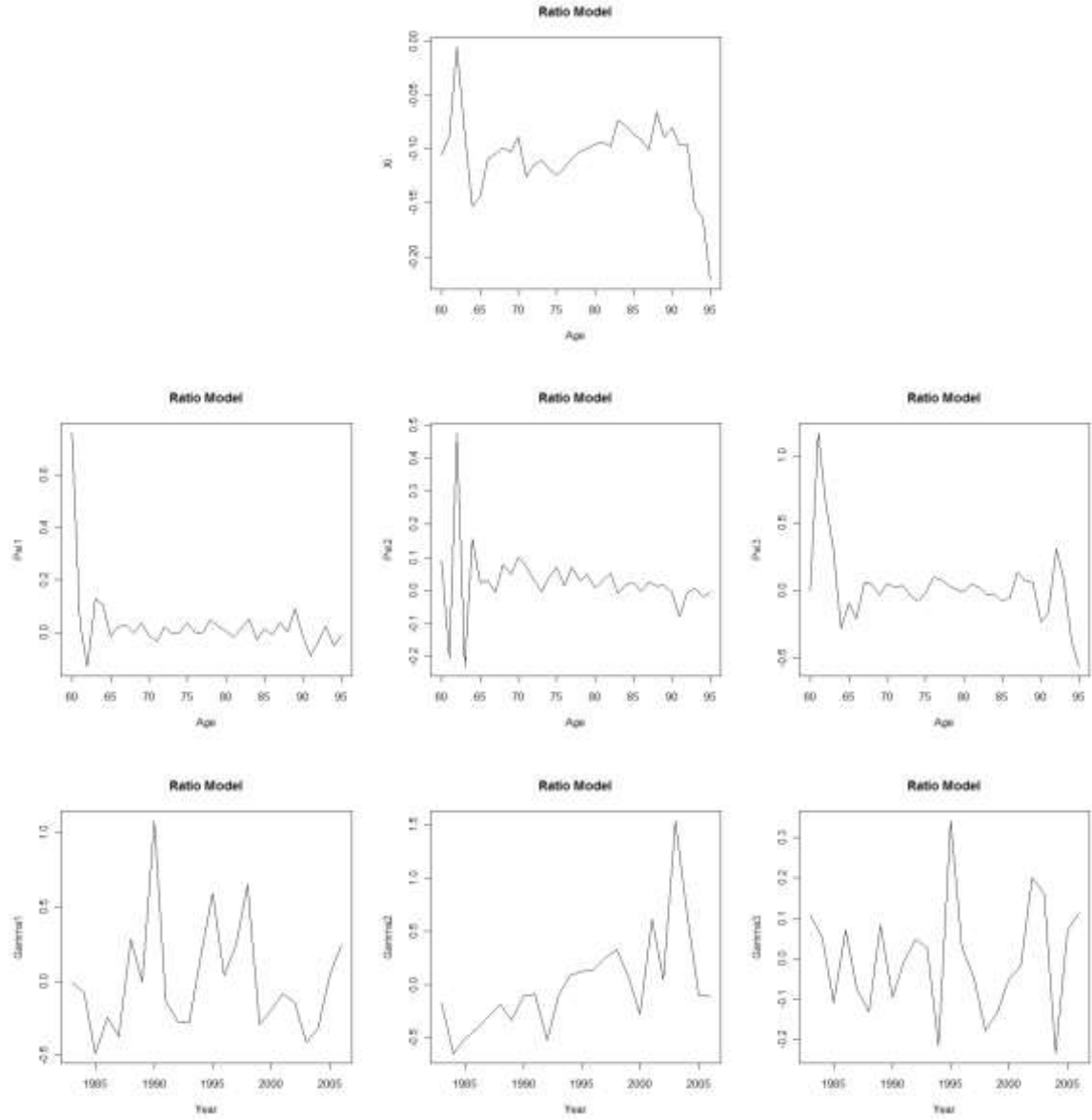
Fig. 5. Parameter estimates of \xi_x (top), \psi_x(j) (middle), and \gamma_t(j) (bottom) of ratio model of PRM for j = 1, 2, 3 (left to right of last two rows).
