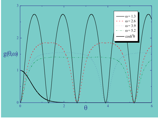
Figure 3: Absolute value squared of minimal form factors g(\theta, \omega) = \lim_{N \rightarrow \infty} |\hat{F}_{\min}(\theta, N)|^2 as functions of the rapidity for different values of \omega and x = 0.1 .
