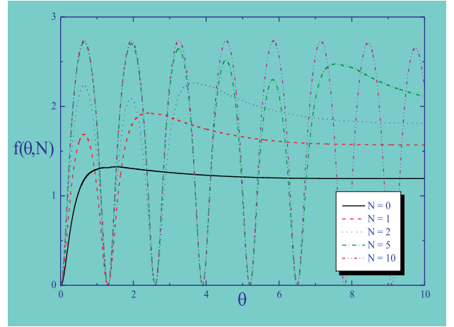
Figure 2: Absolute value squared of the two particle form factors f(\theta, N) = |\hat{F}_2^{\Theta}(\theta, N)|^2 / (2\pi)^2 as functions of the rapidity for different values of N for \omega = 1.3 and x = 0.1 .
