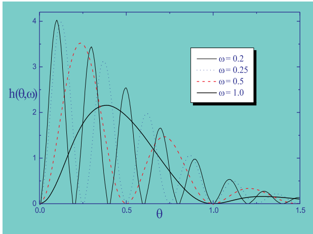
Figure 4: Integrand of equation (25), that is h(\theta, \omega) = \lim_{N \rightarrow \infty} |\hat{F}_{\min}(\theta, N)|^2 / \cosh^4 \theta as a function of the rapidity for different values of \omega and x = 0.1 .
