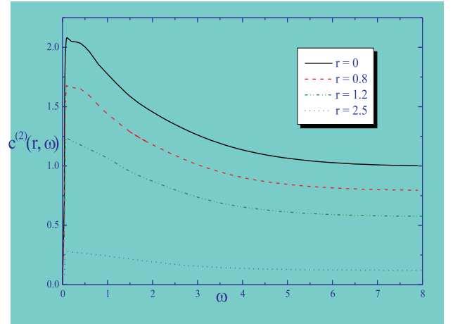
Figure 6: Ultraviolet Virasoro central charge c^{(2)} as a function of \omega .
