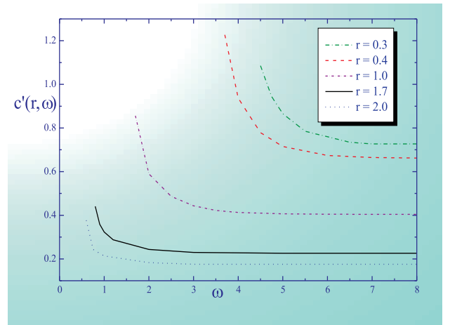
Figure 7: TBA scaling function.
