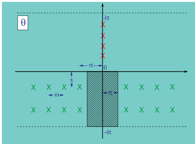
Figure 1: The poles of the blocks \{x\}_{\theta,\ell}^\sigma are the crosses in the sheet -\pi \leq \text{Im } \theta \leq 0 . The crosses on the positive part of the imaginary axis are associated, as usual, with stable particles. For equal masses of the stable particles the threshold (16) is \sigma_t = \text{arccosh}[(3 - \cos \pi x)/(1 + \cos \pi x)] .
