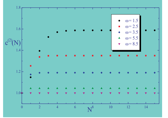
Figure 5: Ultraviolet Virasoro central charge c^{(2)} as a function of N .
