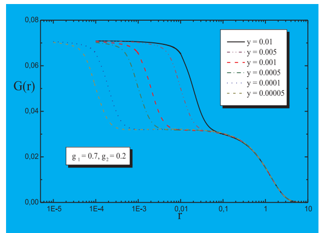
FIG 3: Conductance G for the free Fermion with two defects D_n(\bar{\psi}, \psi) = \bar{\psi}(g_1 + g_2 \gamma^0)\psi at distance y as a function of the inverse temperature m/T .
