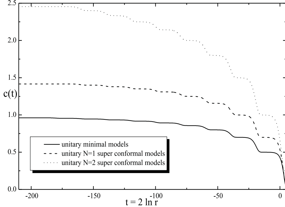
Figure 4: Internal RG flow for the N = 0, 1, 2 unitary minimal models.
