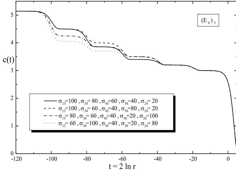
Figure 3: RG flow from q -deformed Virasoro characters.
