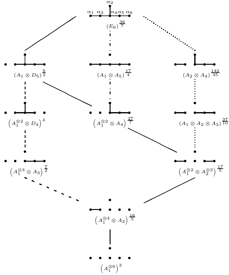
Figure 2: The decoupling of the A_1|E_6 -theory.
