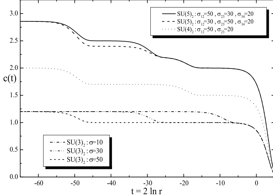
Figure 1: RG flow from q-deformed Virasoro characters.
