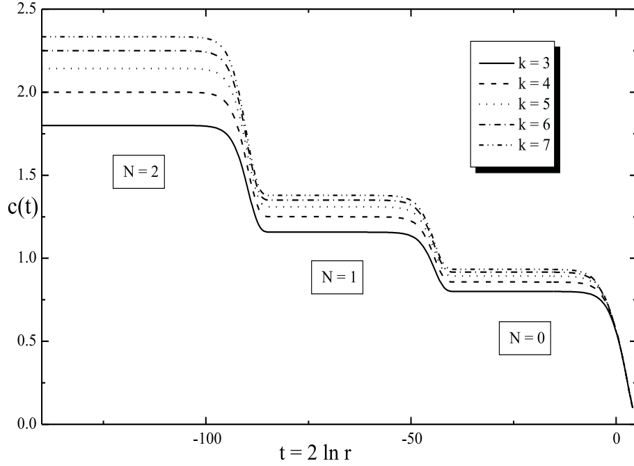
Figure 5: RG flow between N = 0, 1, 2 unitary minimal models.
