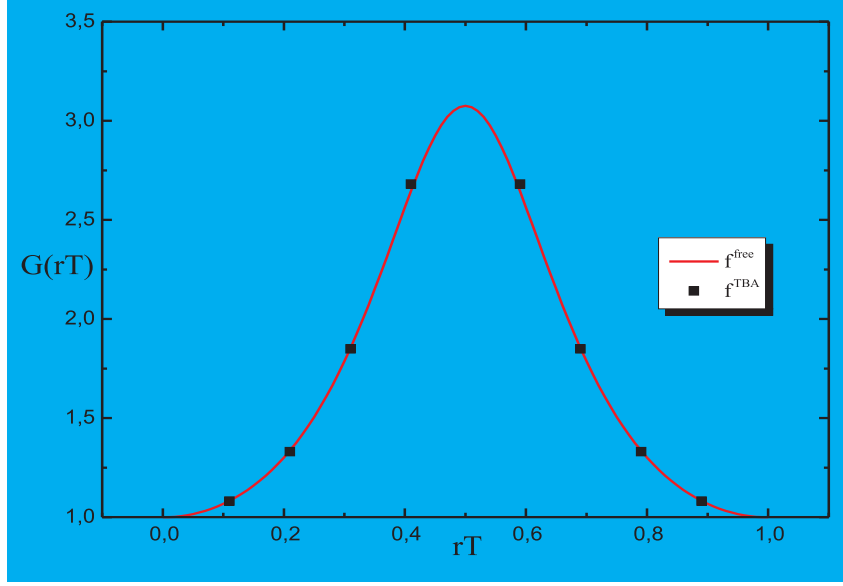
Figure 3: Exact correlation function versus dressed one particle form factor contribution G(rT) := \langle \bar{T}(r) \bar{T}(0) \rangle_{T \neq 0, m=0} / \langle \bar{T}(r) \bar{T}(0) \rangle_{T \neq 0, m=0}^{(1)} .
