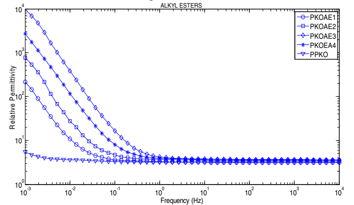
Fig. 4: Real Relative Permittivity of Palm Kernel Oil and its Alkyl Esters.
