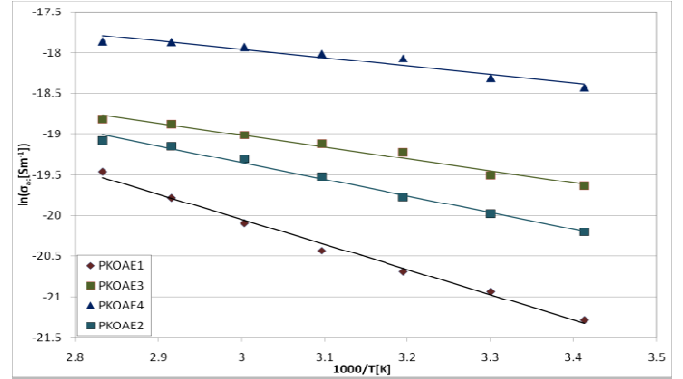
Fig. 7: AC conductivity on Arrhenius Axes (measurement before treatment)
