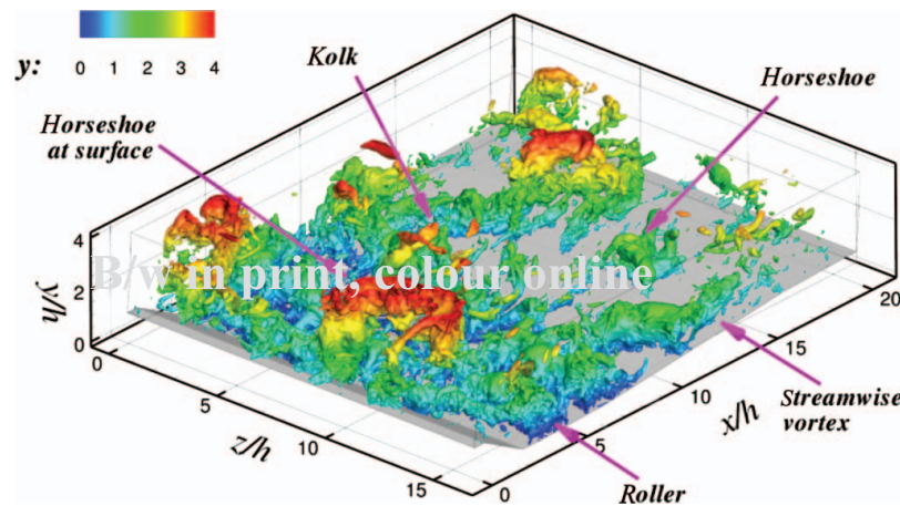
Figure 10. Instantaneous isosurfaces of pressure fluctuation colored with height.
