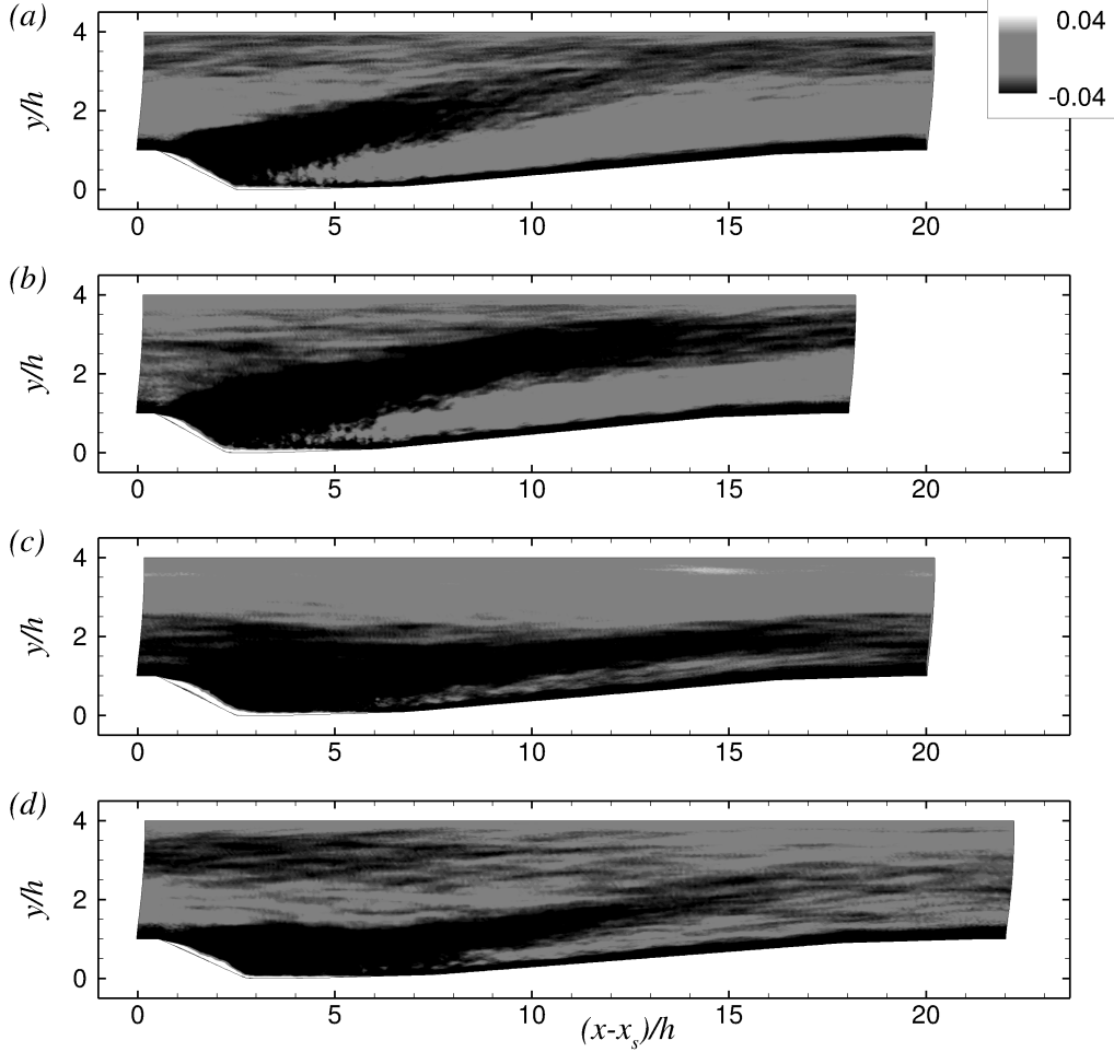
FIGURE 13. Contours of the probability density function of counter-clockwise oriented spanwise eddies minus the probability density function of clockwise oriented spanwise eddies, over (a,b) the lobe and (c,d) the saddle planes of (a,c) the in-phase and (b,d) the staggered crestline alignments.
