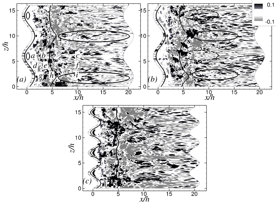
FIGURE 5. Instantaneous streamwise-velocity fluctuations, u' , on a plane 0.05h above the bed; (a) Case 5; (b) Case 11 (c) Case 9. Solid lines are contours of \langle \bar{u} \rangle = 0.0 representing the mean separation and reattachment lines. The ovals highlight regions in which the streamwise vortices cause upwash.
