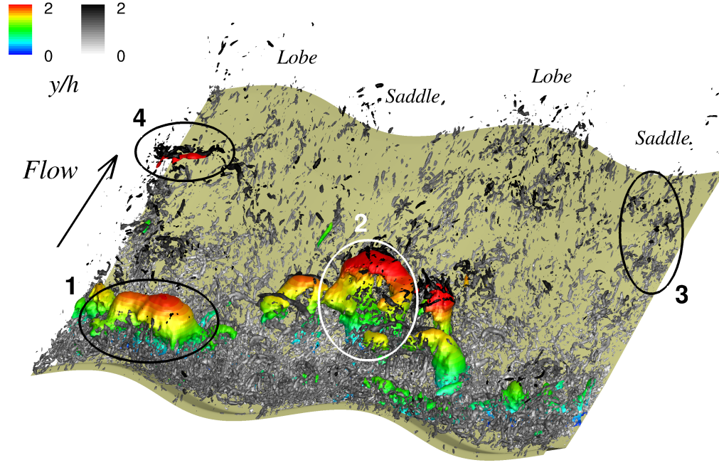
FIGURE 3. Instantaneous flow structures for the in-phase crestline alignment, Case 5. Isosurfaces of pressure fluctuations p'/\rho U_b^2 = -0.061 are coloured by the distance from the bed with rainbow colormap and isosurfaces of the second invariant of the velocity tensor, Qh^2/U_b^2 = 5.29 , are coloured by the distance from the bed with grayscale colormap.
