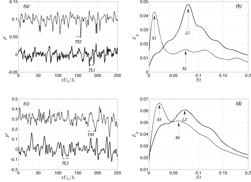
FIGURE 9. (a,c) Time history and (b,d) spectra of local pressure fluctuations near the reattachment point for (a,b) in-phase crestline alignment (Case 5) and (c,d) staggered crestline alignment (Case 11). — Lobe and --- saddle planes.
