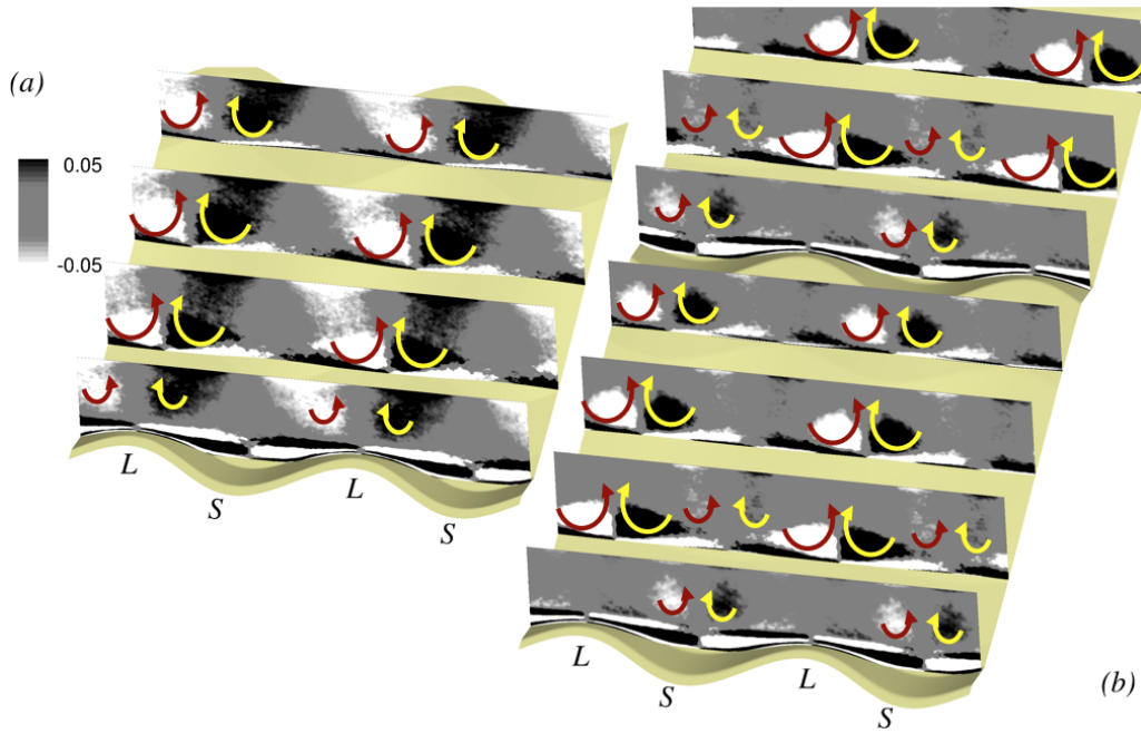
FIGURE 2. Contours of mean streamwise vorticity, \Omega_x h / U_b , for (a) Case 5 and (b) Case 11 on crossplanes at x/h = 2.0, 7.0, 12.0, 17.0, 22.0, 27.0 , and 32.0 . Arrows show the mean secondary flows. “L” represents the lobe and “S” represents the saddle.
