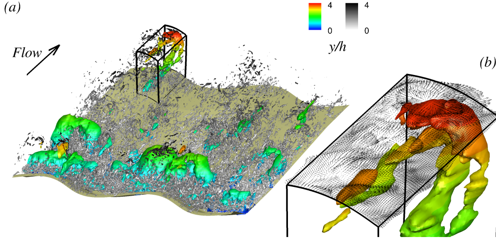
FIGURE 16. Instantaneous flow visualization at tU_b/h = 172.1 . Isosurfaces of pressure fluctuations p'/\rho U_b^2 = -0.03 are coloured by the distance from the bed with rainbow colormap and isosurfaces of the second invariant of the velocity tensor, Qh^2/U_b^2 = 3.8 , are coloured by the distance from the bed with grayscale colormap. (a) Entire flow field; (b) enlargement of the vortex impinging on the surface, and tangent velocity fluctuation vectors at the surface.
