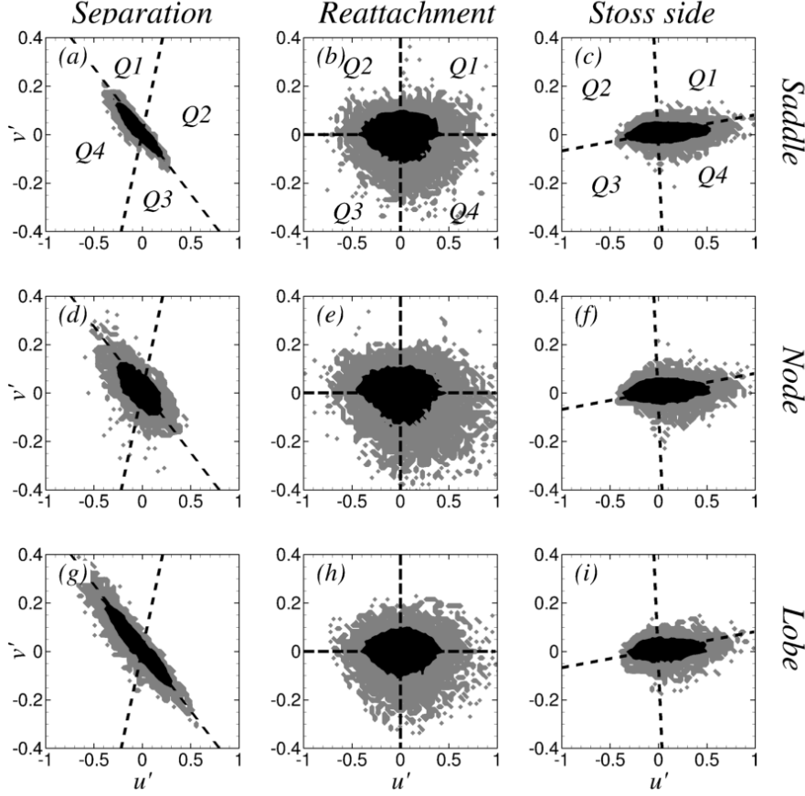
FIGURE 8. Joint probability density contours of u' and v' at the points indicated in Figure 5(a). --- represents the alignment of the bed. Contour levels represent density of 0.01 and 0.11; the points are the same as those in Figure 7.
