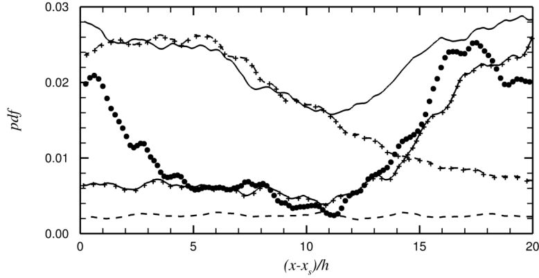
FIGURE 17. Probability of strong boils over a time h/U_b at the free surface. Lines: in-phase; lines and symbols: staggered; \bullet 2D (Omidyeganeh & Piomelli 2011). — Lobe and --- saddle planes.
