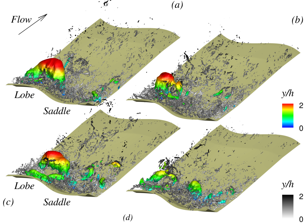
FIGURE 11. Instantaneous flow structures for the staggered crestline alignment at four instants of the time-series shown in Figure 9(a). Only half of the channel is shown. (a) tU_b/h = 110.4 , (b) tU_b/h = 125.6 , (c) tU_b/h = 174.7 , and (d) tU_b/h = 194.6 . Isosurfaces of pressure fluctuations p'/\rho U_b^2 = -0.076 are coloured by the distance from the bed with rainbow colormap and isosurfaces of the second invariant of the velocity tensor, Qh^2/U_b^2 = 7.6 , are coloured by the distance from the bed with grayscale colormap.
