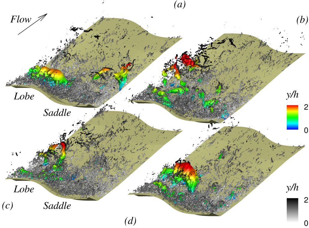
FIGURE 10. Instantaneous flow structures for the in-phase crestline alignment at four instants of the time-series shown in Figure 9(a). Only half of the channel is shown. (a,b) Vortices shed over the lobe, (a) tU_b/h = 178.2 , (b) tU_b/h = 190.4 . (c,d) Events over the saddle affected by vortices shed over the lobe, (c) tU_b/h = 145.6 , and (d) tU_b/h = 156.9 . Isosurfaces of pressure fluctuations p'/\rho U_b^2 = -0.076 are coloured by the distance from the bed with rainbow colormap and isosurfaces of the second invariant of the velocity tensor, Qh^2/U_b^2 = 7.6 , are coloured by the distance from the bed with grayscale colormap.
