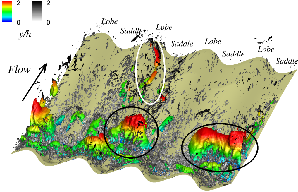
FIGURE 4. Instantaneous flow structures for the in-phase crestline alignment, Case 9. Isosurfaces of pressure fluctuations p'/\rho U_b^2 = -0.061 are coloured by the distance from the bed with rainbow colormap and isosurfaces of the second invariant of the velocity tensor, Qh^2/U_b^2 = 5.29 , are coloured by the distance from the bed with grayscale colormap.
