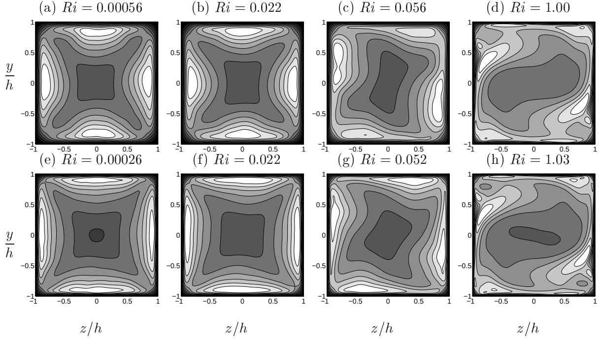
FIG. 11: The same as Fig. 7 but for the streamwise r.m.s. velocity \sqrt{u'^2} represented in gray scales (white and black shows the maximum and minimum value, respectively). The maximum values of \sqrt{u'^2}/u_b , are (a) 0.66, (b) 0.67, (c) 0.66, (d) 0.63, (e) 0.65, (f) 0.64, (g) 0.61, (h) 0.63, respectively. (a-d) Re_b = 3000 , (e-h) Re_b = 4400 .
