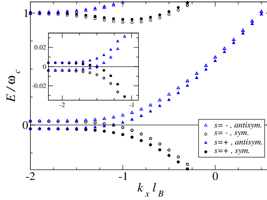
Fig. 3 Dispersion relation E_{s,\pm}(k_x) of a semi-infinite graphene sheet with an armchair edge at y=0 , obtained numerically from Eq. 30. We use \lambda=0 , B=15 T, \Delta=6 meV, and the + ( - ) sign is for the symmetric (antisymmetric) valley combination in Eq. 30. Inset: Same for \Delta=0.3 meV.
