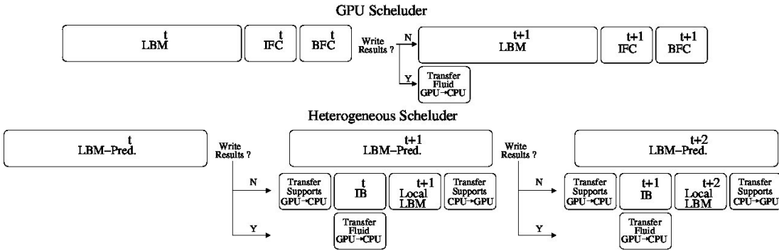
Figure 2: GPU (top) and CPU-GPU Heterogeneous (bottom) implementations.
