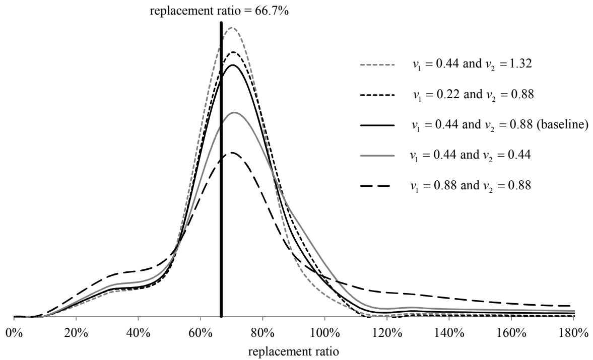
Figure 11 – Effect on the replacement ratio of changing curvature parameters, \nu_1 and \nu_2
