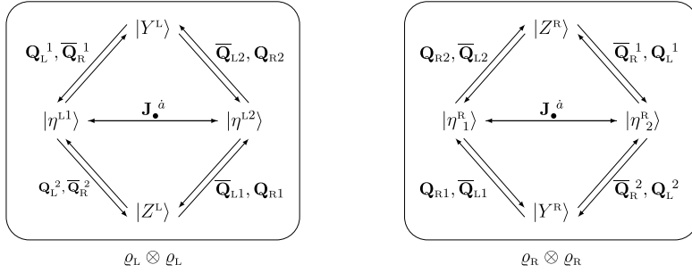
Fig. 1. The massive excitations and their transformation properties under \mathcal{A} . The left and right panel depict the left and right representations respectively. The bosons Z^{L,R} are excitations on \text{AdS}_3 while Y^{L,R} are excitations on S^3 . Note that the massive fermions \eta^{L\dot{a}}, \eta^{R\dot{a}} are charged under \mathfrak{su}(2)_\bullet . The tensor products below each diagram indicate how each representation can be obtained from the short fundamental representations of \mathfrak{su}(1|1)_{\text{c.e.}}^2 introduced in Section 3.1.3.
