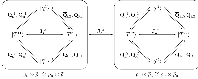
Fig. 2. The massless excitations transform in two irreducible representations of \mathfrak{psu}(1|1)_{\text{c.e.}}^4 , which form a doublet under \mathfrak{su}(2)_o . Each of these representation can equivalently be taken to be the massless limit of a left or a right representation with a fermionic highest-weight state. For definiteness, here we take both of them to be given by left representations. Below each \mathfrak{psu}(1|1)_{\text{c.e.}}^4 diagram we indicate how each representation can be obtained from one of two (left or right) isomorphic tensor products of fundamental \mathfrak{su}(1|1)_{\text{c.e.}}^2 representations, see Section 3.1.3.
